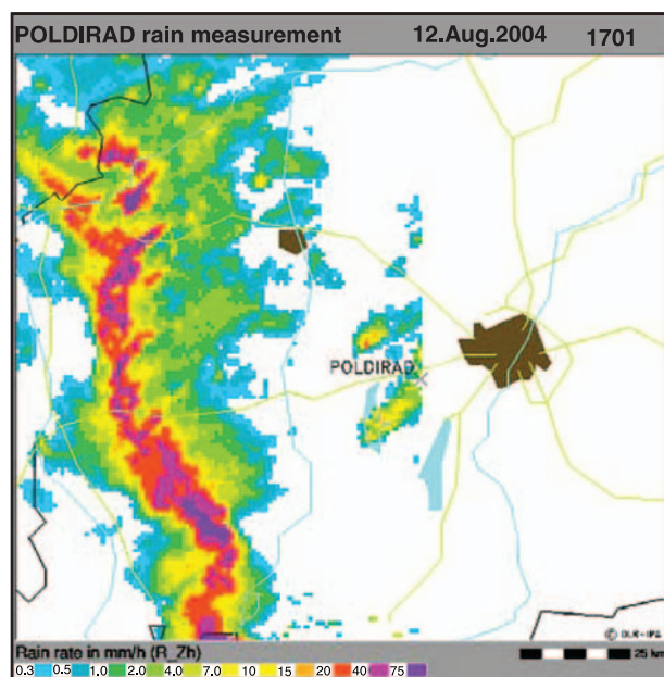
Fig. 7. Instantaneous rainrate (mm/h) in the sector west of Munich (large patch), determined from polarimetric measurements at 1701 UTC on 12 August 2004; radar beam elevation: 1^\circ ; pixel size: 1 \text{ km} \times 1 \text{ km}
