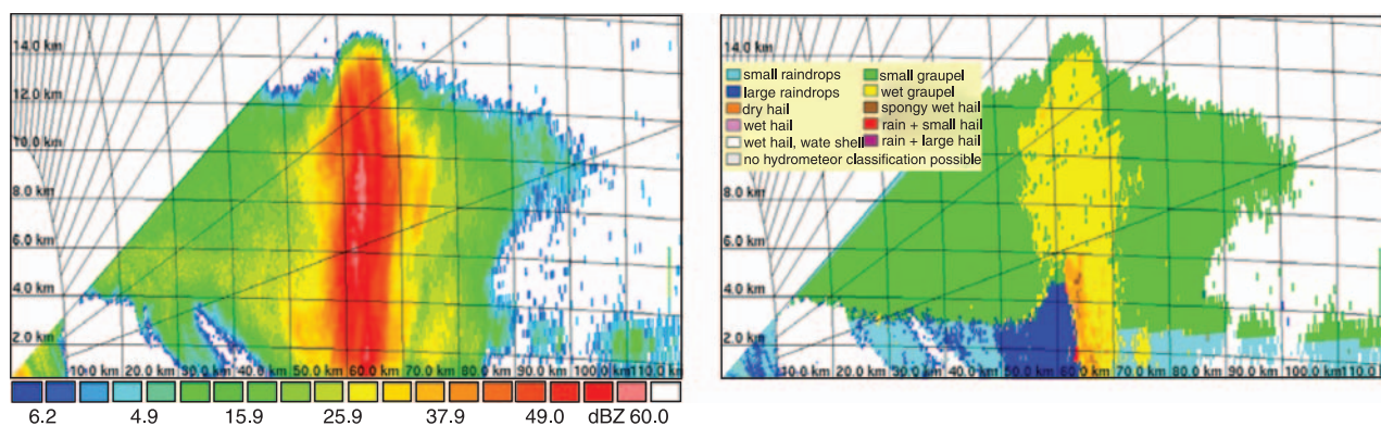
Fig. 6. Cross-section at 1658 UTC on 12 August 2004 towards SW ( 240^\circ ) through an approaching thunderstorm with the polarimetric radar POLIDRAD at DLR Oberpfaffenhofen: reflectivity (left) and hydrometeor classification (10 classes) from various combinations of polarimetric data (right)
