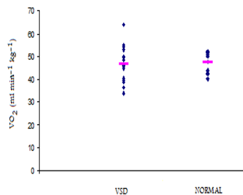
Fig. 1 (b) Ventricular Septal Defect vs. Normal; Maximal Oxygen Uptake: (ml min -1 kg -1 )
