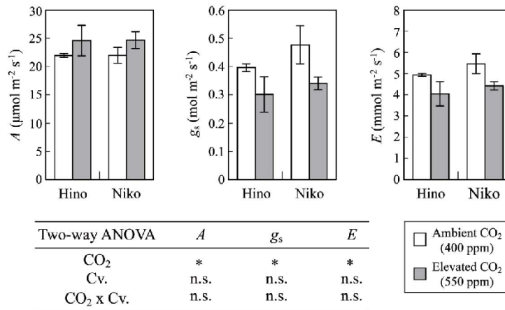
Fig. 3. Effects of elevated CO 2 on the net photosynthetic rate ( A ), stomatal conductance ( g_s ), and transpiration rate ( E ) in the flag leaf of two Japanese cultivars of rice in late August 2018. Hino: Hinohikari (heat-sensitive); Niko: Nikomaru (heat-tolerant). Each value represents the mean of three chamber replicates, and error bars represent the standard deviations. Two-way analysis of variance (ANOVA): * p < 0.05 , n.s. = not significant.
