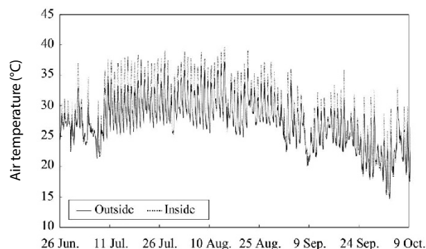
Fig. 1. Time course of temperature outside and inside open-top chambers (OTCs) during the experimental period from 26 June to 9 October 2018. Number of hours exceeded the 35°C outside and inside the OTCs during the period were 39 and 240, respectively.
