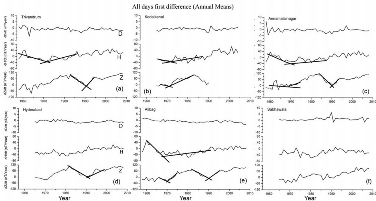
Fig. 8. Plot of the first difference of annual mean values of declination (D), horizontal component (H), and vertical component (Z), for all days at (a) Trivandrum, (b) Kodaikanal, (c) Annamalaiagar, (d) Hyderabad, (e) Alibag, and (f) Sabhawala, from 1958 to 2009.
