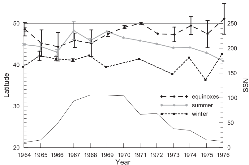
Fig. 11. Same as Fig. 10 but for solar cycle 20.
