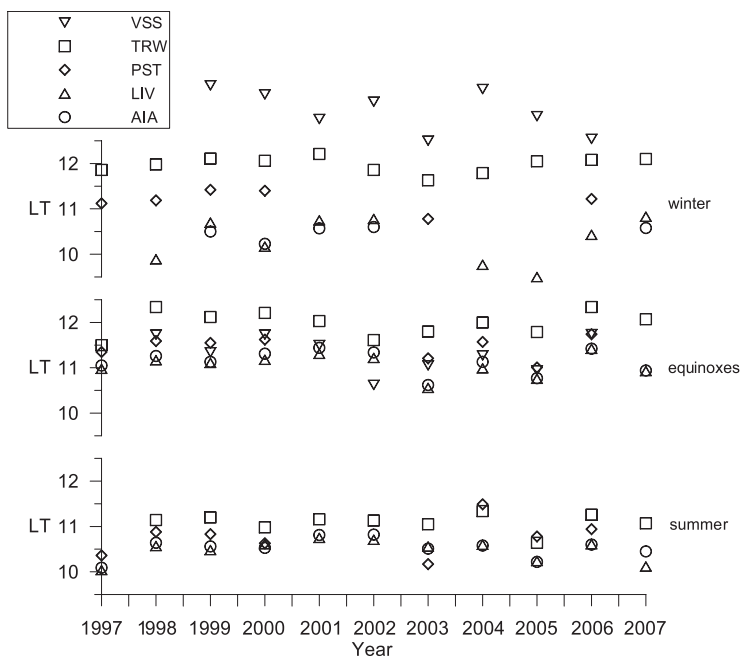
Fig. 8. Time at which the variation of D passes through zero for each season and year at each observatory.
