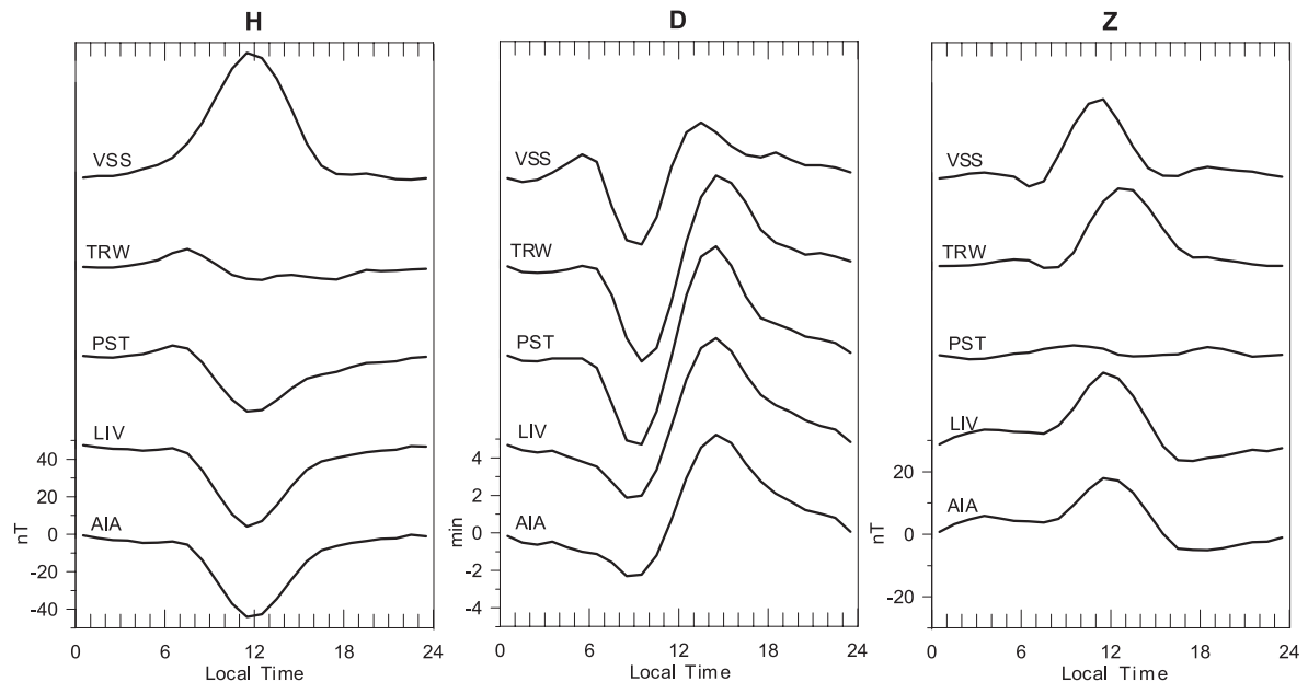
Fig. 6. Averages for the equinoctial season daily variations at the different observatories for 1999.
