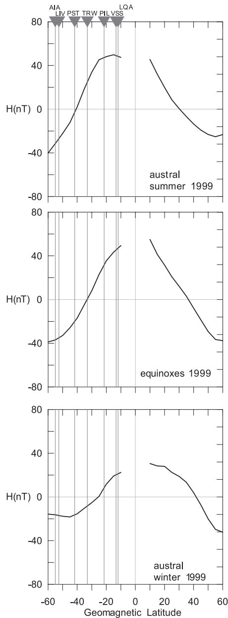
Fig. 7. Typical H variation for the average of five International Quiet Days of each month for 1999 when the variation of D passes through zero at different locations (every 5^\circ and excluding the points closest to the geomagnetic equator) as a function of geomagnetic latitude from the CM4 model. Positions of the observatories used in the analyses are given according to their geomagnetic latitude.
