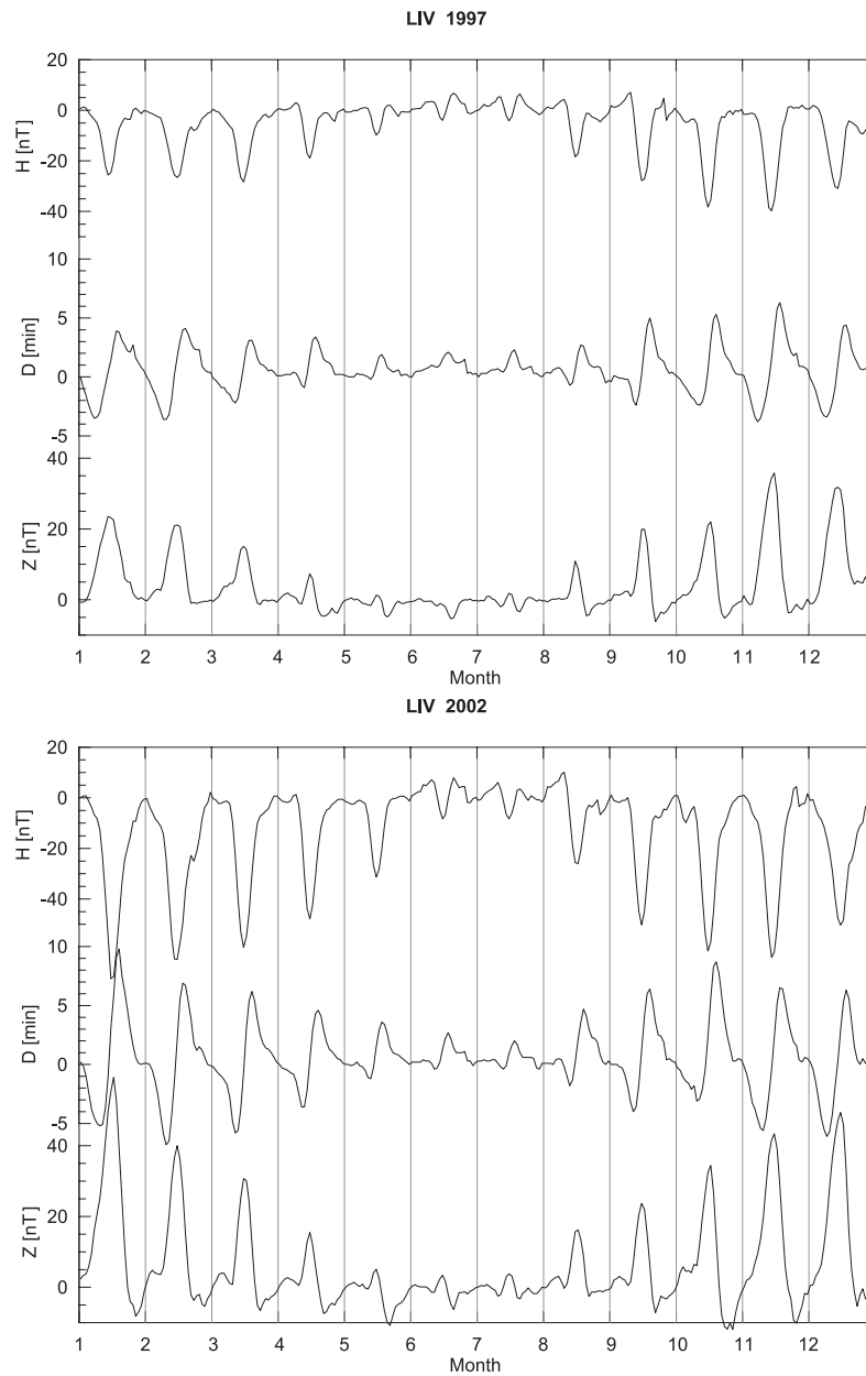
Fig. 3. Daily LT variations at LIV for a low- (top) and a high (bottom)-activity year. These variations were obtained from hourly mean values averaged over the five quietest days of each month.
