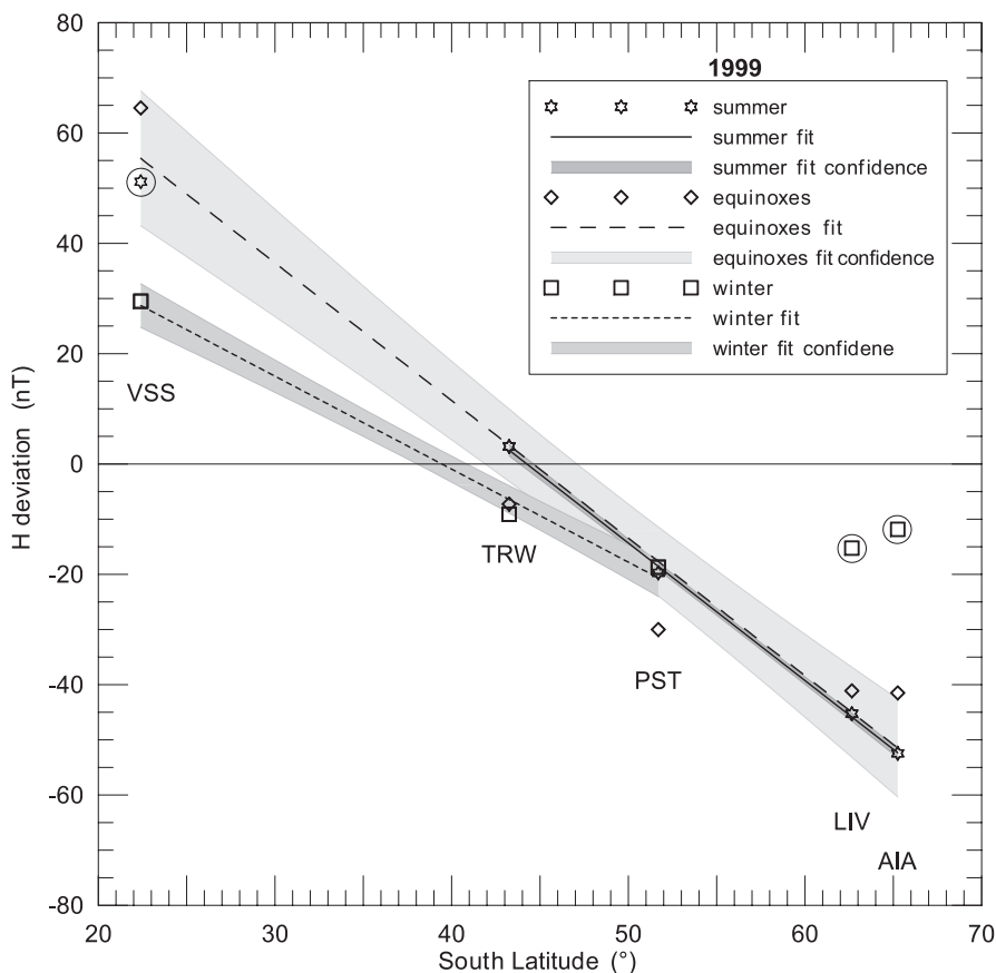
Fig. 9. Plot of variation of H versus observatory latitude used for the determination of the focus latitude of the ionospheric current system by least squares fits for each season of 1999. The standard uncertainties of the fits are also displayed as grey shadings. Symbols for AIA and LIV for winter and VSS for summer are encircled to indicate that they were not considered for the fit.
