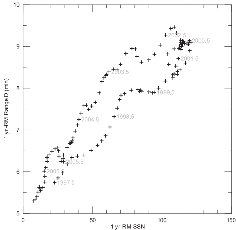
Fig. 5. One-year running mean of the monthly mean values of the daily range of D at LIV versus the corresponding values of the solar sunspot number (SSN). Labels every 12 months indicate the time evolution.
