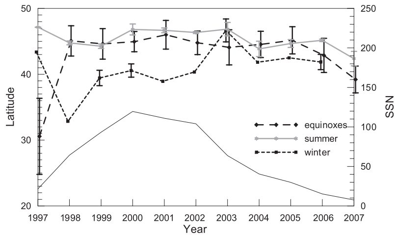
Fig. 10. Evolution of the determined focus latitude of the ionospheric current system for each year and season of solar cycle 23 (with their error bars), along with the yearly averaged SSN.
