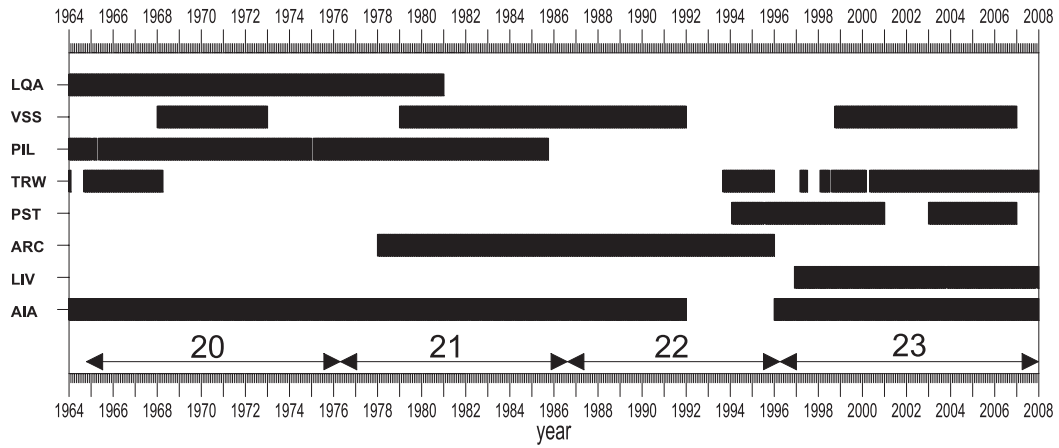
Fig. 2. Histogram showing the availability of data from the different stations with respect to the last four solar cycles.
