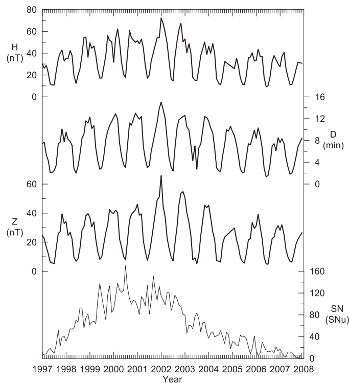
Fig. 4. Time evolution of the daily amplitude of the S_q variation at LIV and of the monthly averaged solar sunspot number (SN).
