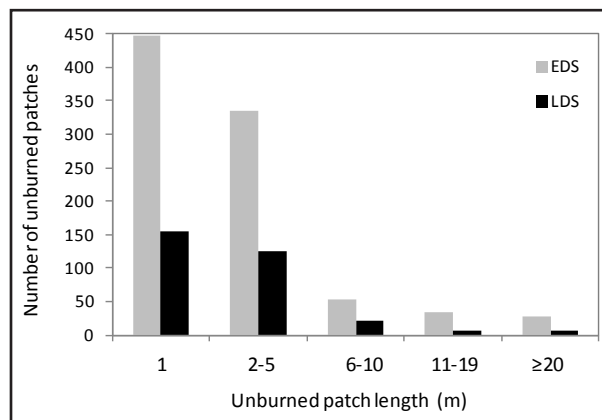
Figure 4. Frequency distribution of unburned patch size for the early dry season (EDS) and late dry season (LDS).
