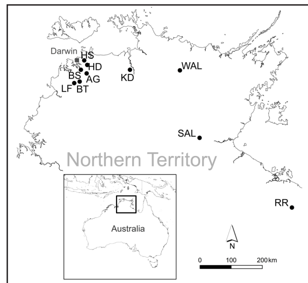
Figure 1. Location of the study areas in the Northern Territory, Australia.
