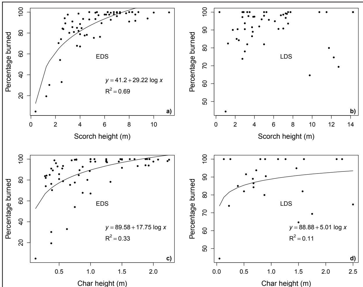
Figure 6. Scatter plots of the percentage burned and scorch height (m) in the a) early dry season (EDS), and b) late dry season (LDS); scatter plots of the percentage burned and char height (m) in the c) early dry season (EDS), and d) late dry season (LDS), for data aggregated at 200 m. The solid line is the best logarithmic curve fitted to the data. Since the logarithm of scorch height and percentage burned for LDS were uncorrelated ( R^2 \approx 0 ), the curve is omitted.
