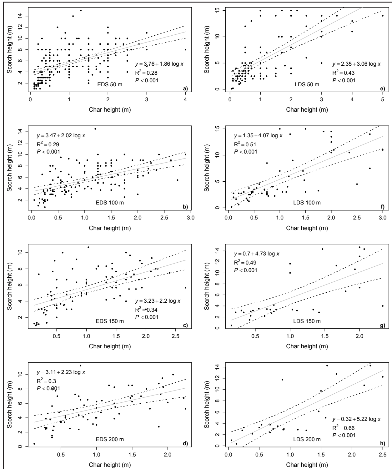
Figure 5. Regression analysis between char and scorch heights in the early dry season (EDS) for data aggregated at a) 50 m, b) 100 m, c) 150 m, and d) 200 m, and in the late dry season (LDS) for data aggregated at e) 50 m, f) 100 m, g) 150 m, and h) 200 m. Dashed lines correspond to a 95% confidence band around the regression line.
