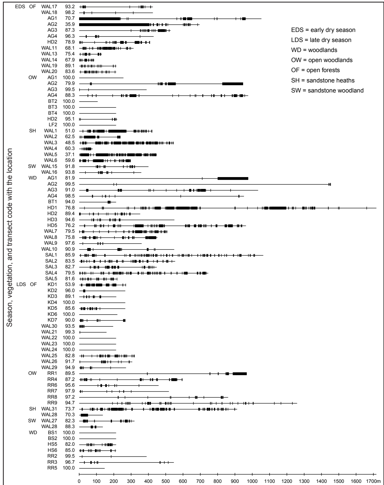
Figure 2. Transect profiles of unburned points (black vertical lines) grouped by season and vegetation type. Each transect containing more than one vegetation type was segmented by vegetation type, and for two-way ANOVA only its longest segment was kept. Next to each transect is the percentage of the transect that burned.
