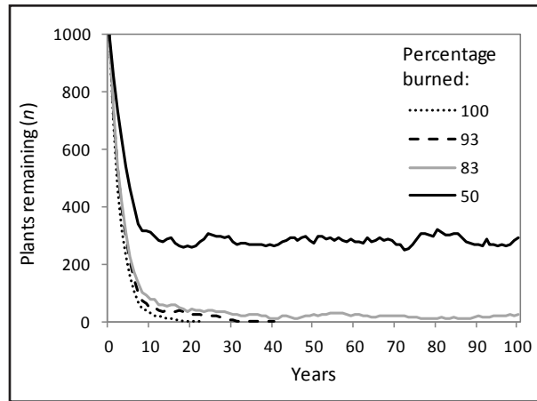
Figure 7. Plant survival according to different percentage burned (100%, 93%, 83% and 50%) with ability to recolonise after seven years without fire.
