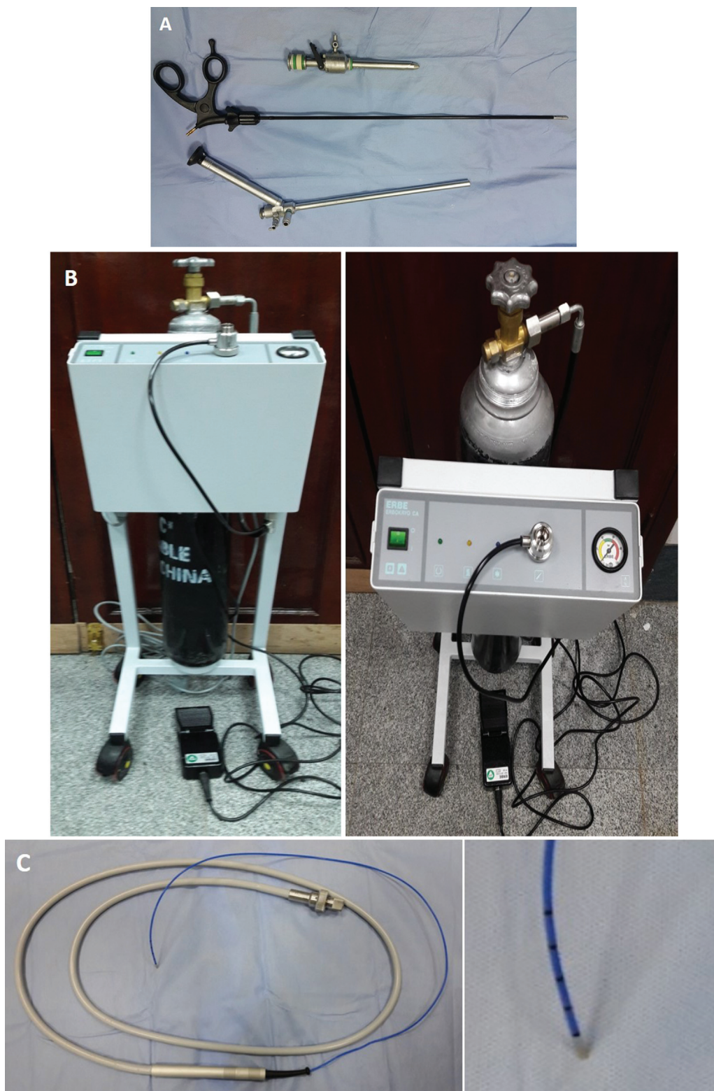
(a) Thoracoscopy instruments (Karl-Storz, Germany) including trocar and cannula; rigid biopsy forceps and single-entry rigid telescope for adults. (b) Erbe Cryo unit (Germany). (c) Flexible cryoprobe (Erbe, Germany).
