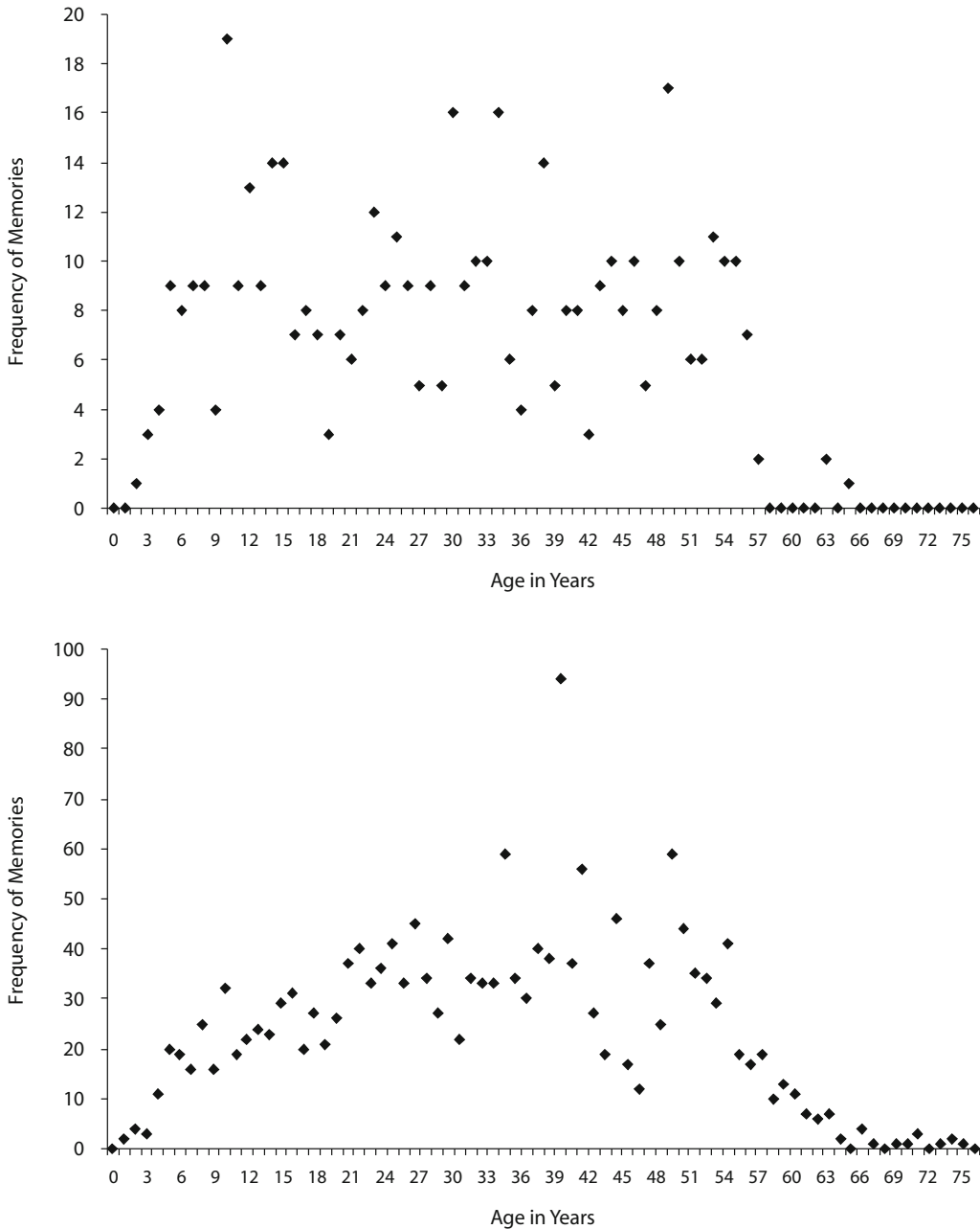
Figure 1. Studies 1 (upper panel) and 2 (lower panel): Graph to show distribution of memories across the life span.
