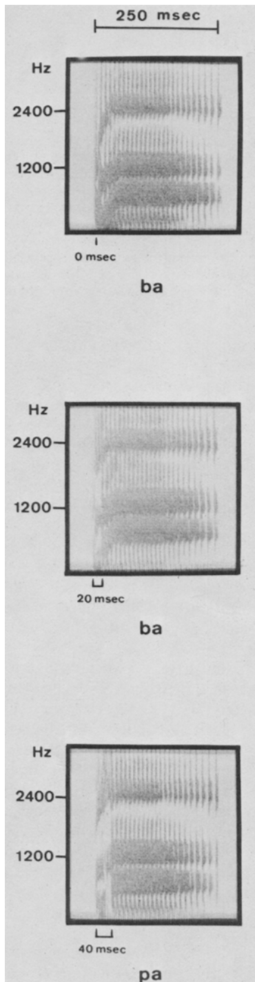
Fig. 1. Sound spectrograms of the speech stimuli 0 VOT [ba], 20 VOT [ba], and 40 VOT [pa].
