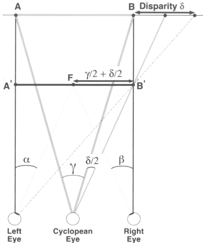
Figure 2. The perceived horizontal dimension difference between two distinct depth planes: Schematic top view of an observer fixating point F in the plane of line A'B' . This line occludes line AB . A and B are only visible monocularly. For the observer, A looks as if it is aligned with A' , and B looks as if it is aligned with B' (Erkelens, Muijs, & van Ee, 1996). If the observer were to use the retinal local signs ( \alpha and \beta ) directly to estimate the dimension that is occluded in the background ( \gamma ), he or she would overestimate this dimension by an amount that is equal to the disparity between the fixation plane and the background. Note that this statement is true for fixation in any depth plane. If fixation is behind the plane of interest, the sign of the disparity is reversed. From an operational point of view, it is convenient to use a single vantage point (the so-called cyclopean eye) from which the stereoscopic visual world is viewed, rather than using the views of two eyes. This cyclopean eye is located midway on the line that connects the nodal points of the eyes. But note that, mathematically speaking, the location of the single vantage point is essentially irrelevant for the above-derived statements.
