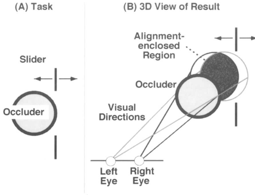
Figure 1. Task and results according to Erkelens, Muijs, and van Ee (1996). (A) Schematic view of the subject's perception of the scene in the experiment of Erkelens et al. An occluding disk was hovering in front of a background. In fact, the occluder was monocularly invisible because it was presented as a random-dot pattern relative to an identical background random-dot pattern (Julesz stereogram). A binocularly visible slider was presented in the background, and the task of the subject was to align the slider with the rightmost (or leftmost) part of the disk's rim. One slider was visible at a time. The slider consisted of two parts that were segments of an (invisible) line. The slider was oriented either vertically (shown at the right side of the rim) or horizontally (not shown). (B) An artist's conception of the results of Erkelens et al. The figure shows a slider when it was perceived to be aligned with the rightmost part of the disk's rim. Erkelens et al. found that the horizontal dimension of the occlusion (in fact, the dark area in the background constituted by the slider alignments at the leftmost and rightmost parts of the occluder's rim) is smaller than the vertical dimension of the occlusion.
