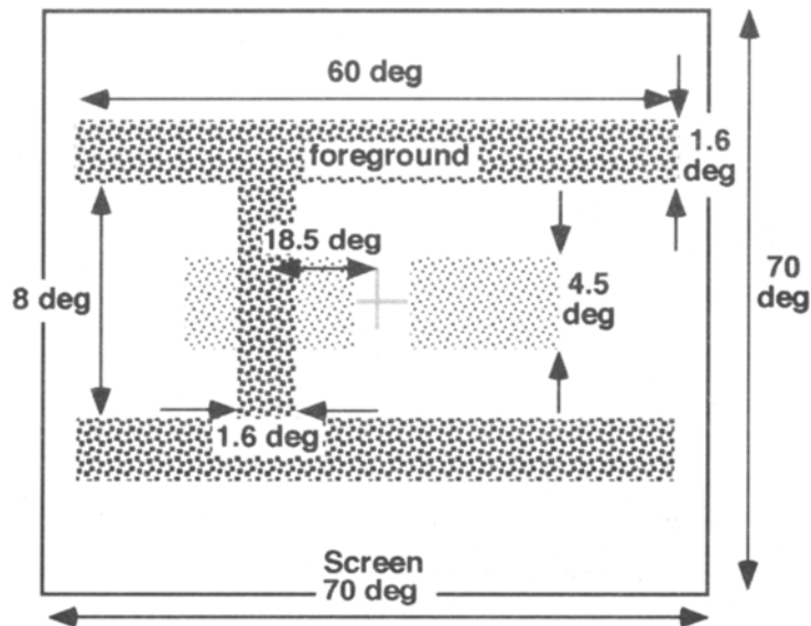
Figure 10. Stimulus of Experiment 4. The vertical dimension of the rectangles was fixed at 4.5^\circ . The horizontal dimension of the left rectangle was 28.0^\circ , 29.8^\circ , or 31.6^\circ . The horizontal dimension of the right rectangle varied randomly between 86% and 114% of the dimension of the left rectangle. The subjects were instructed to discriminate whether the rectangle behind the occluder was wider and narrower than the nonoccluded rectangle. The center of the left (right) rectangle was always presented 18.5^\circ to the left- (right-) hand side of the center of the screen (marked by the gray cross). Whenever the vertical foreground bar (size, 1.6^\circ \times 8^\circ ) was present, it was presented 18.5^\circ to the left-hand side of the screen (that is, on top of the center of the left rectangle). The bar was part of a foreground pattern that was 60^\circ wide. The boundaries of the screen (size, 70^\circ \times 70^\circ ) and the cross in the center were not visible. Although the figure shows different textures, the textures in the experiment were identical (Julesz stereogram). There was no background present.
