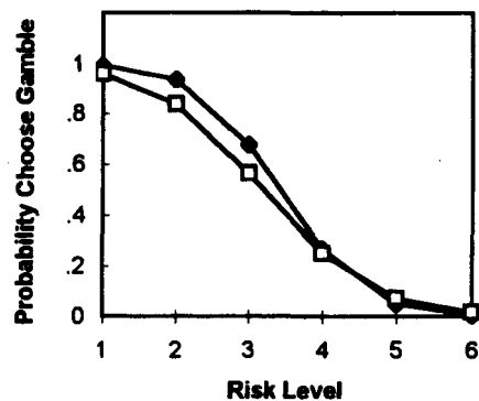
Figure 1. The left three panels show the probability of taking an additional card by the participants as a function of risk level. The top, middle, and bottom panels are for low, moderate, and high computer card levels. In all panels, there is a backward-S-shaped curve as risk level increases, and the time pressure curve is flatter than the no time pressure curve. Furthermore, there is a crossover interaction between the curves for the time pressure and no time pressure conditions in each of the panels. These effects are moderated by the computer card level, but only for the no time pressure condition. The right three panels show the predictions of the model for choice probability under the same experimental conditions. The steeper curve represents the predictions when the inhibitory threshold is set to a high criterion and the bound is increased, and the flatter curve represents the predictions when the inhibitory threshold is set to a low criterion (under time pressure) and the bound is smaller. The precise quantitative form of the curves depends on specific parameter values estimated from the data, but the crossover interaction pattern and the effect of the computer card level is a parameter-free prediction of the model.
