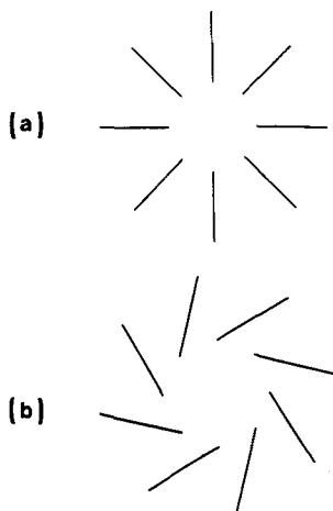
Figure 10. (a) Bright illusory circle induced perpendicular to the ends of the radial lines. (b) Illusory circle becomes less vivid as line orientations are chosen more parallel to the illusory contour. Thus, illusory induction is strongest in an orientation perpendicular to the ends of the lines, and its strength depends on the global configuration of the lines relative to one another. From Perception and Pictorial Representation (p. 182) by C. F. Nodine & D. F. Fisher (Eds.). New York: Praeger, 1979. Copyright 1979 by Praeger. Adapted by permission.
