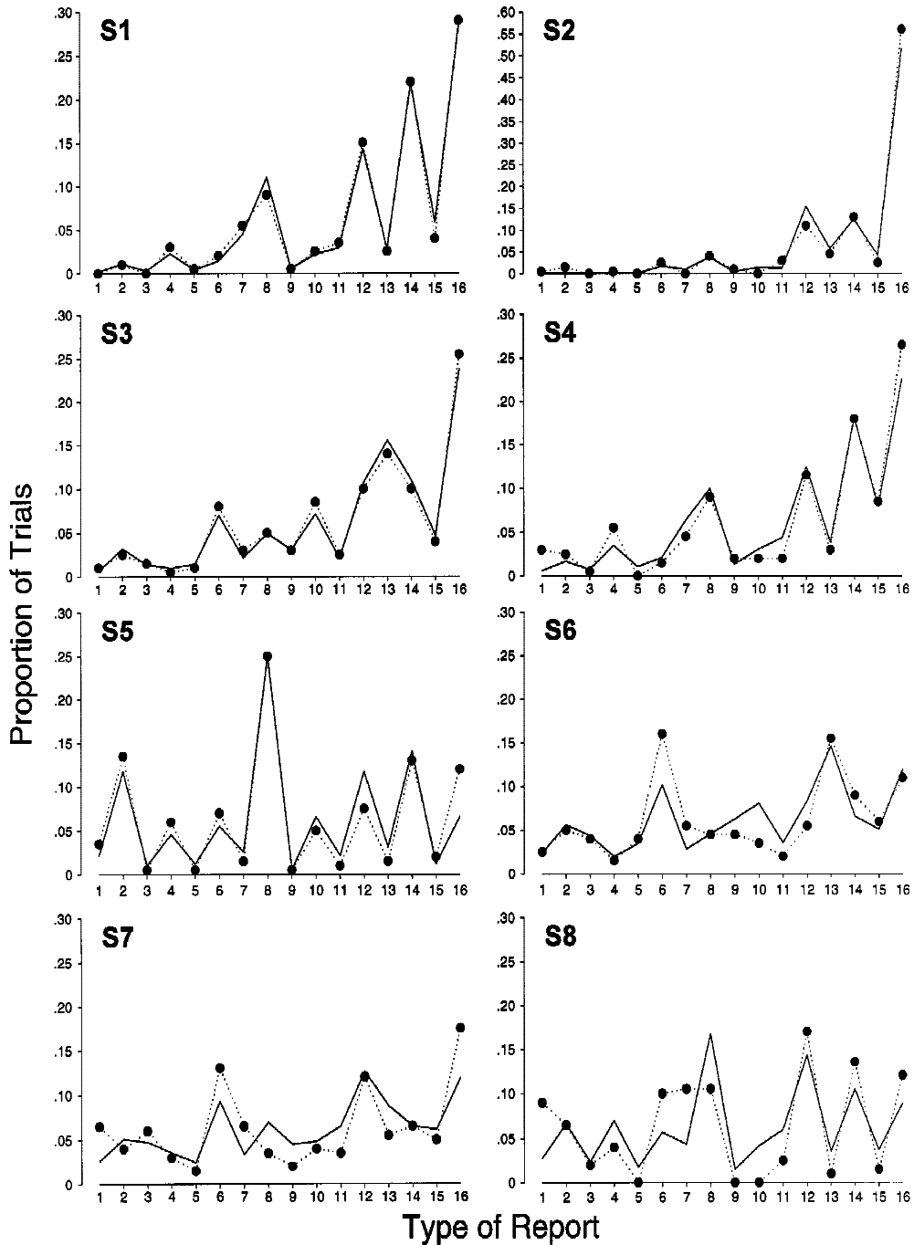
Figure 1. Observed and predicted probability distributions of reports of pairs of colored shapes across 16 types of report for Observers S1–S8. Observed probabilities are shown by solid circles connected with dotted lines. Predicted probabilities are indicated by unmarked points connected with unbroken lines. The predictions were derived from observed probabilities (in Table 1) of correct identification of the left shape, the left color, the right shape, and the right color, respectively, by assuming mutual independence between reports of the four features. The 16 types of report are defined in Table 2.
