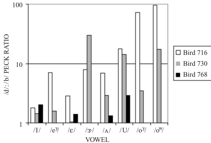
Figure 3. Reanalysis of the quail peck rate categorization data from Kluender et al. (1987) showing higher /d:/b/ peck ratios for back vowels /U, o y , o w / in comparison with front vowels /i, e y , ε/. Diphthongs are ordered relative to the F2 of the initial vowel, which would determine the pattern of F2 onset transition.
