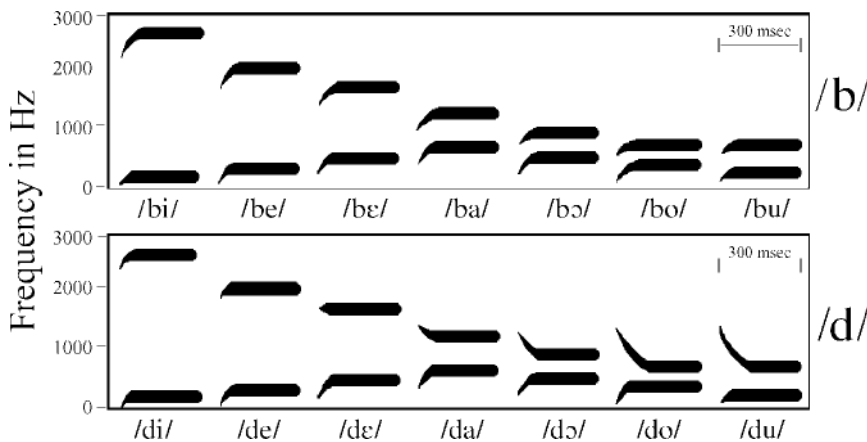
Figure 4. Schematized spectrograms depicting the F1 and F2 onset transitions for /b/ versus /d/ in the context of several different vowels. From “Acoustic Loci and Transitional Cues for Consonants,” by A. Liberman, C. Delattre, and F. Cooper, 1955, Journal of the Acoustical Society of America , 27, 769-773. Copyright 1955 by Acoustical Society of America. Adapted with permission.
