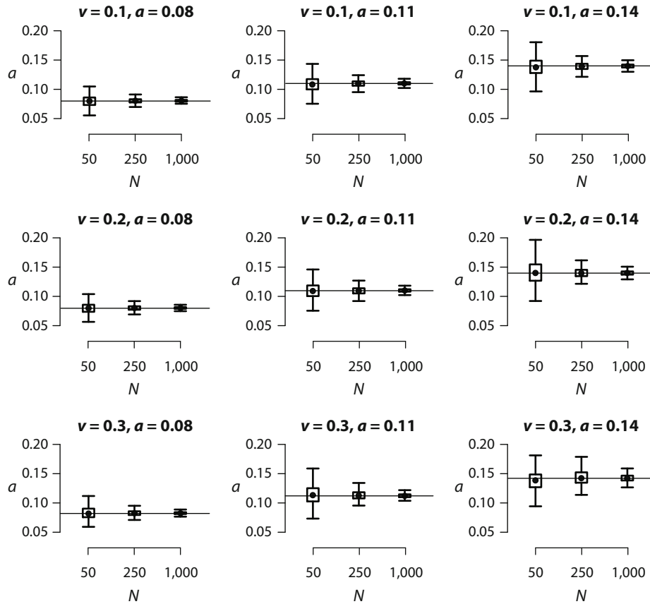
Figure 7. Boundary separation parameter recovery for the EZ-diffusion model. Each panel corresponds to a different combination of data-generating parameter values for \nu and a . The data-generating values for boundary separation are indicated by horizontal lines. Each box-plot is based on 1,000 replications.
