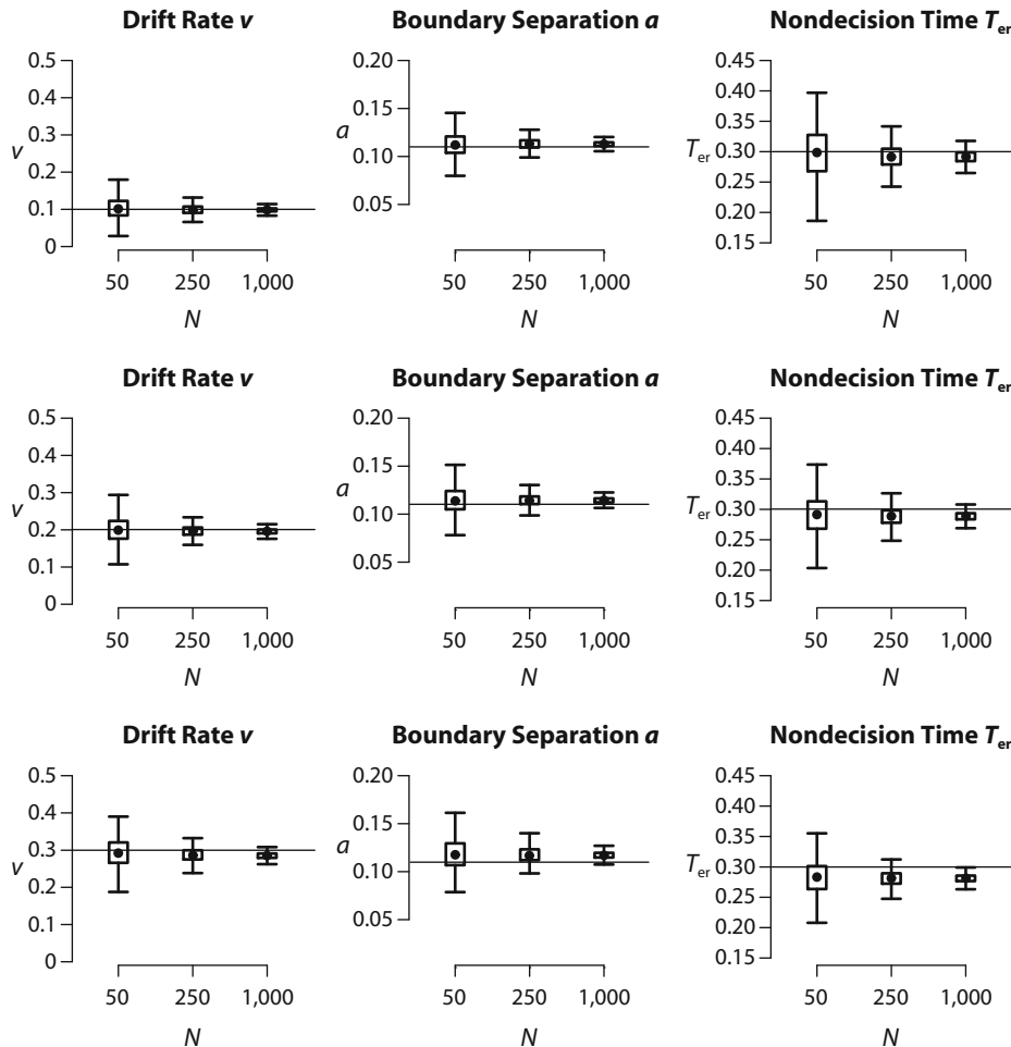
Figure 9. Parameter recovery for the EZ-diffusion model under misspecification, with the data-generating process affected by across-trials variability in nonddecision time. The uniform distribution of nonddecision time has a range of 0.200 sec, which is at the extreme end of what is observed in practice (Ratcliff & Tuerlinckx, 2002). Boundary separation a was fixed at an intermediate value of 0.11, and the mean of the nonddecision time T_{er} was fixed at 0.300. Panels in the top, middle, and bottom rows were generated using drift rate values of 0.1, 0.2, and 0.3, respectively. Data-generating parameter values are indicated by horizontal lines. Each box-plot is based on 1,000 replications.
