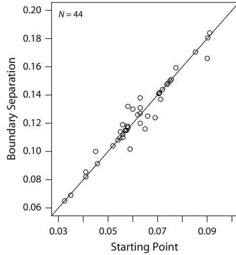
Figure 3. The relationship between starting point and boundary separation as encountered in previous research. The solid line has a slope of 2, suggesting that in many situations the starting point is about equidistant from the two response boundaries.
