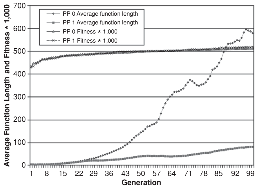
Figure 2. Average function length and fitness (*1,000) by generation, with (PP 1) and without (PP 0) the minimal parsimony pressure of 1%. This figure shows that even a small parsimony pressure (penalty for long functions) can have a marked effect on average function length, while having little effect on fitness. In order to show both fitness and length on the same graph, we have multiplied fitness values (correlations with the predictor) by 1,000. These data are from the ON × FREQ problem discussed in Example 1.
