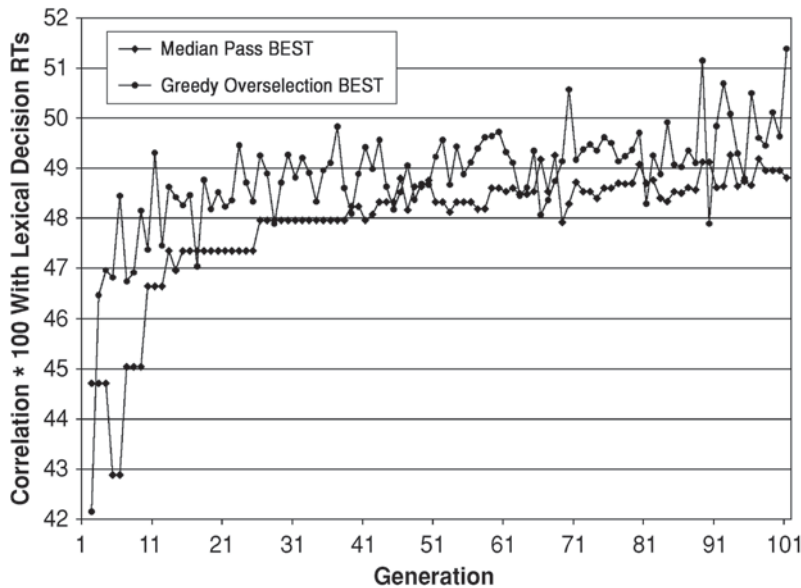
Figure 5. Two typical evolutionary runs of the best evolved predictor, by generation, for the two selection schemes offered in NUANCE. Median Pass selection with age weighting is always less erratic, but Greedy Overselection (which cannot benefit from age weighting) almost always performs slightly better at predicting variance. The dependent variable in this example is lexical decision RTs using two predictors (see Example 1 in the text).
