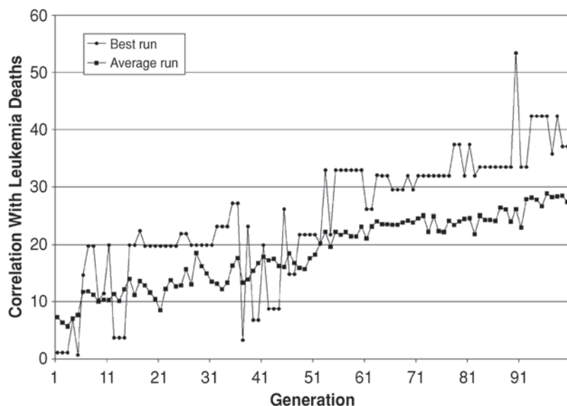
Figure 6. Best and average of the 10 NUANCE runs for Example 2, predicting leukemia deaths from cigarette consumption.
