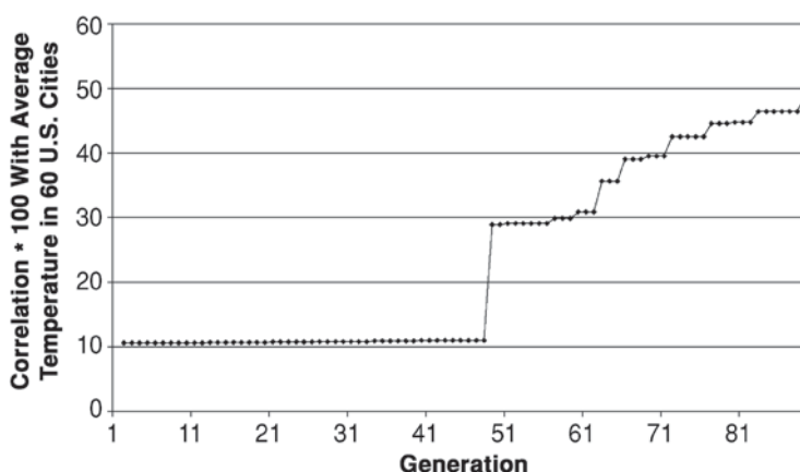
Figure 1. A NUANCE fitness curve, using Median Pass selection, illustrating the danger of over-reliance on the shape of the fitness curve as a measure of whether or not one has run sufficient generations. This problem used a data set from DASL, at lib.stat.cmu.edu/DASL/Datafiles/SMSA.html , to estimate the average January temperature in 60 U.S. cities from average rainfall in those cities. The fitness curve is almost perfectly flat with a correlation of approximately .11 for 47 generations, which might lead one to conclude that no better solution was possible. However, a breakthrough at generation 48 led to substantial and thereafter increasing improvement on this early estimate. This illustrates why it is a good idea to run as many generations as possible.
