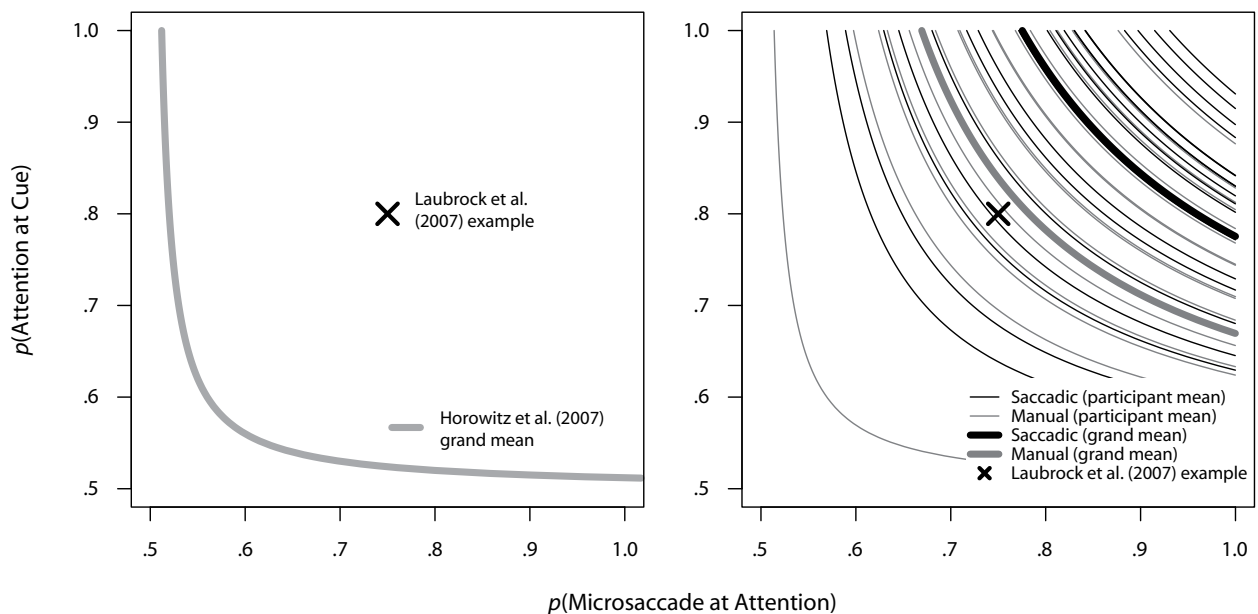
Figure 2. Each curve represents the observed probability of target-incongruent microsaccades given valid cues, and shows how this constrains the possible values for the unknown probabilities that attention followed the spatial cue ( y -axis) and that microsaccades followed attention ( x -axis). Curves are constructed following the analysis presented in Laubrock et al. (2007) and Horowitz, Fencsik, et al. (2007); see the text for details. (Left) Reconstruction of Horowitz, Fencsik, et al. (2007) and Horowitz, Fine, et al. (2007) results. (Right) New data. Each thin curve represents a single subject's probability, based on first microsaccades occurring 200–400 msec after cue presentation. Curve color distinguishes between saccadic (black) and manual (gray) responses. Thick lines represent mean probabilities across subjects. Assuming probability matching for attention following a cue ( p = .80 ) and an intermediate probability for microsaccades following the direction of attention ( x = .75 ), the manual-response curve would nearly pass through the point labeled “prediction by Laubrock et al. (2007),” which was included to facilitate comparison with Figure 1 from Horowitz, Fencsik, et al. (2007, p. 368; note that the point there erroneously exchanged coordinates). After visual comparison, only 1 of our subjects (represented by the curve in the lower left corner) produced a cue congruency effect on microsaccade direction that was as small as the average reported by Horowitz, Fencsik, et al. (2007).
