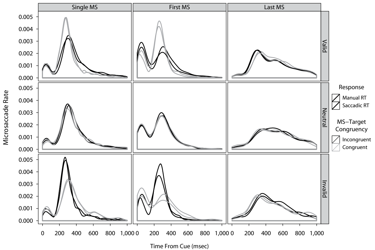
Figure 4. Microsaccade rates across the cue–target interval for target-congruent (gray lines) and target-incongruent (black lines) microsaccades broken down by type of microsaccades (panel columns: single, first of several, last of several), cue validity (panel rows: invalid, neutral, valid), and response modality (manual: thin lines; saccadic: thick lines). Note that target-incongruent rates for invalid cues (bottom row of panels) reflect cue-congruent rates. Thus, cues induce a pronounced peak in microsaccade rate at around 200 msec in the cue–target interval. Graph produced with ggplot (R Development Core Team, 2009; Wickham, 2009). MS, microsaccade.
