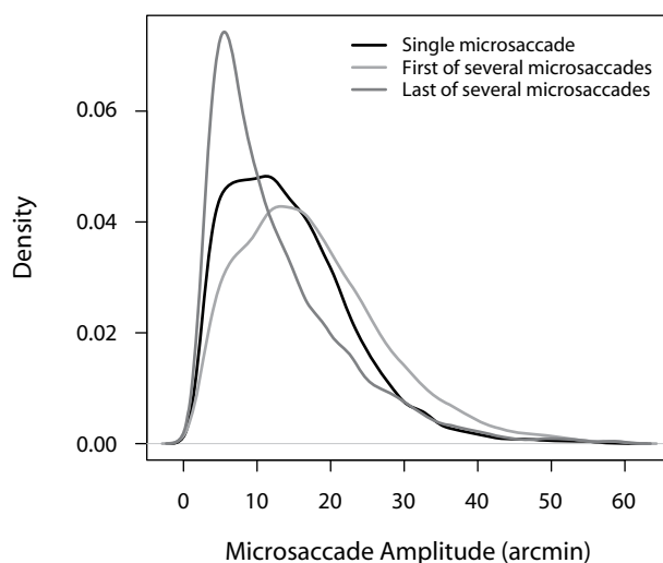
Figure 3. Distributions of microsaccade amplitudes broken down by type of microsaccade (single, first of several, last of several). Densities are collapsed across response modality because their shape was very similar.
