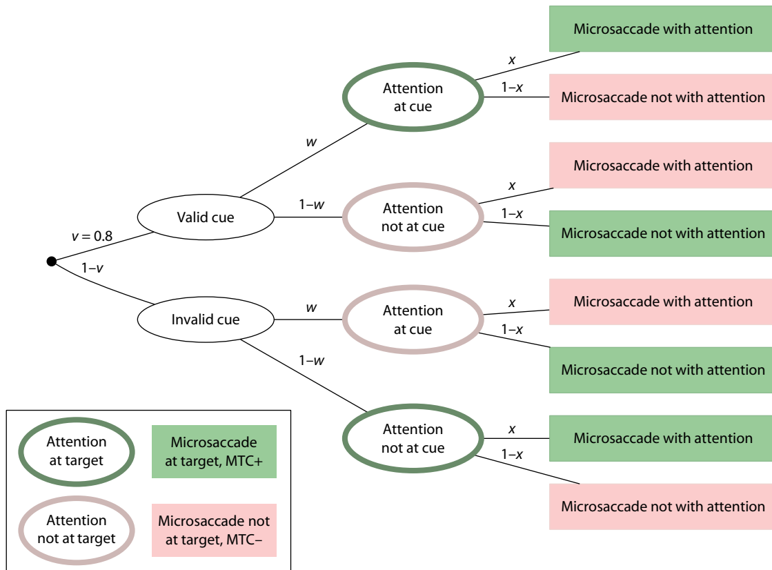
Figure 1. Multinomial tree model about the relation between the direction of spatially cued attention, cue validity, and direction of microsaccades. Neutral cues are omitted to avoid clutter. Validity for direction cues was fixed at v = .80 . The parameter w captures assumptions about attentional strategies—that is, about the probability that attention is indeed shifted in accordance with the cue; the range of reasonable values is between w = v (probability matching) and w = 1.00 (optimal attention shifts). The legend in the lower left corner explains the shape and color codes: Colors classify attention (ovals) or microsaccades (rectangles) with respect to the target; the dark gray and light gray colors indicate shifts toward and away from the target, respectively. At the behavioral level, we can only observe whether microsaccades are target congruent (dark gray rectangles) or target incongruent (light gray rectangles), because we cannot directly observe where attention is shifted. For example, on valid-cue trials (upper branch), we can only observe whether a microsaccade is directed at the target (dark gray rectangles) or not (light gray rectangles), but not whether attention is directed at the target (dark gray oval) or not (light gray oval). Hence, observed microsaccade–target congruency contains a mixture of instances involving attention at the target and away from the target. However, the observed probabilities constrain the possible values of the latent probabilities x and w , because they are the sum of the products of the path probabilities leading to the rectangles of the given color. We are primarily interested in determining boundaries for x , the probability that the direction of attention determines the direction of microsaccades. These could indicate, for example, no relation ( x = .50 ), an intermediate relation ( x = .75 ), or a deterministic link ( x = 1.00 ). MTC, microsaccade–target congruency.
