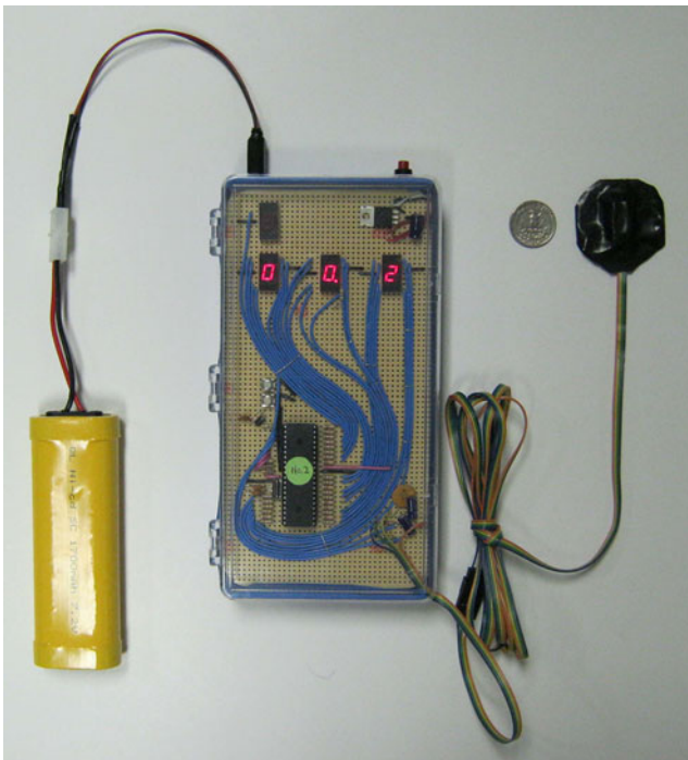
Fig. 6 Photograph of a prototype digital hand inclinometer
