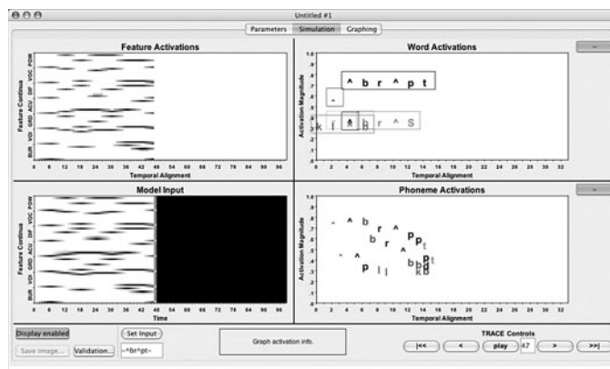
Figure 2. The jTRACE simulation panel.
