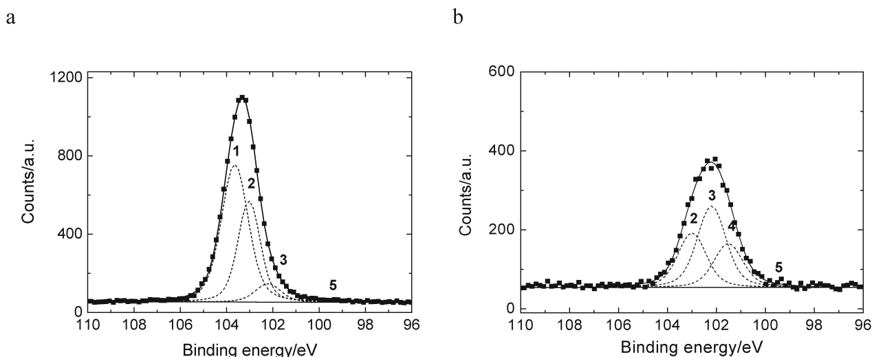
Fig. 7. Deconvolution of high resolution XPS spectra of the doublet subtracted Si2p of Si wafer (a) and DMAN-S modified wafer (b). ■ – Si wafer experimental (a), DMAN-S-Si experimental (b); fit envelope (solid line) (a, b); 1 – SiO 2 , 2 – Si(–O) 3 , 3 – Si–O–Si, 4 – Si(–OR) x , 5 – Si 0 .
