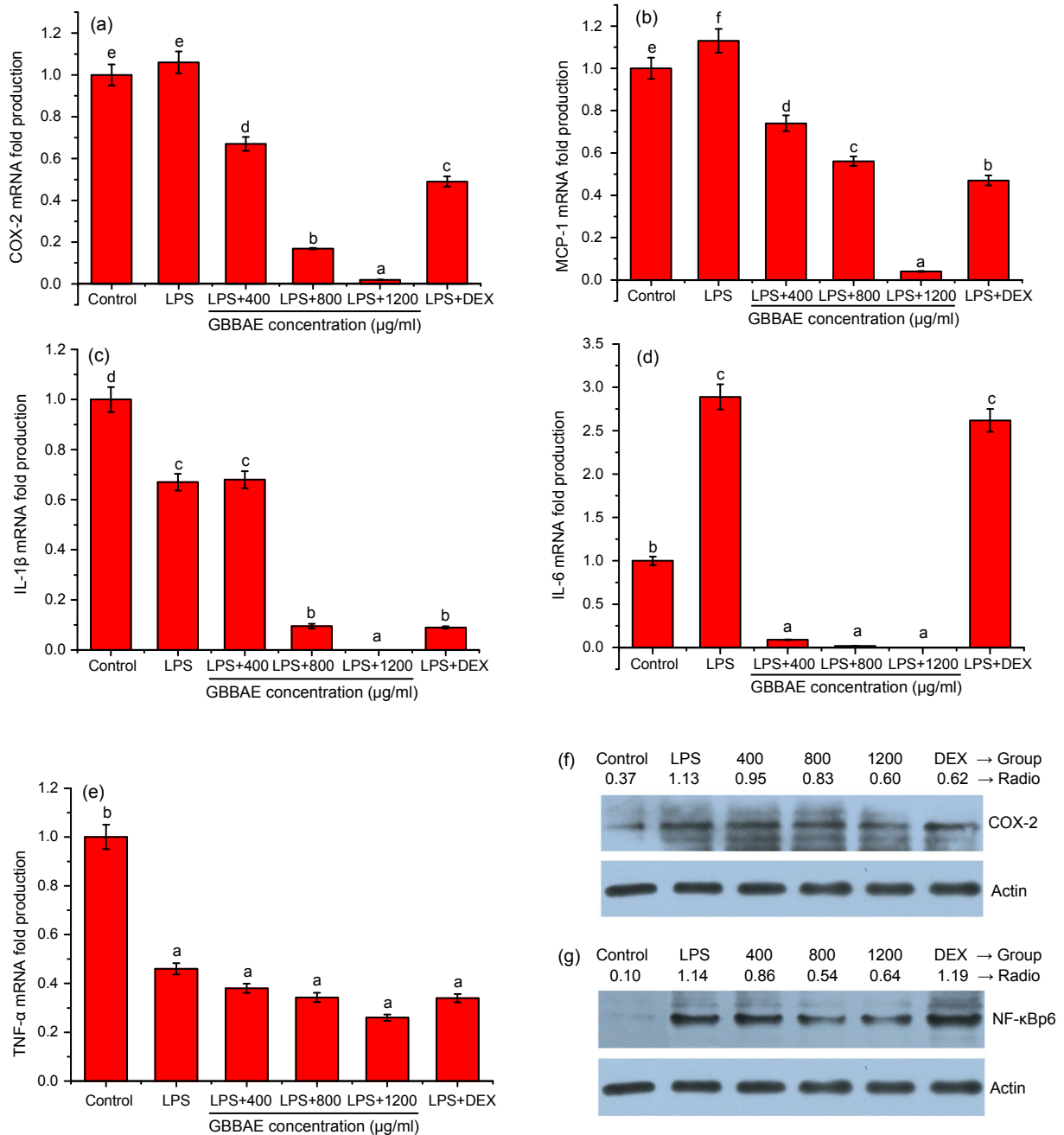
Fig. 5 Effects of GBBAEs on mRNA expression levels of COX-2 (a), MCP-1 (b), IL-1 \beta (c), IL-6 (d), and TNF- \alpha (e) and on the protein expressions of COX-2 (f) and NF- \kappa Bp6 (g) in LPS-stimulated murine RAW 264.7 cells
