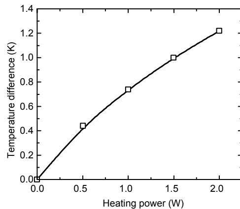
Fig. 5 Calibration of the second thermal bridge
