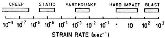
Fig. 1 Magnitudes of strain rates that can be imposed on concretes in compression, classified by Bischoff and Perry [1] according to loading cases which can induce each strain rate. Copyright 1991 RILEM Publications
