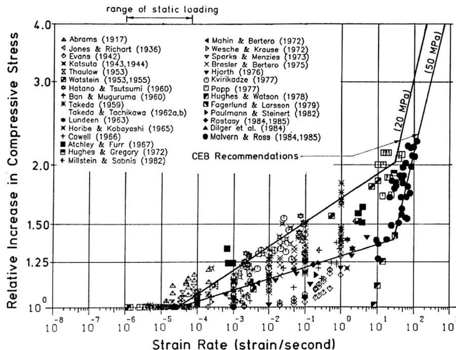
Fig. 2 Influence of strain rate on compressive strength of concretes, along with the 1988 CEB recommendations [7]. Reproduced from [1], Copyright 1991 RILEM Publications
