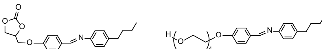
Fig. 4 Structure of MBBA derivatives, 4-butylphenyl)imino)methyl)phenoxy)methyl)-1,3-dioxolan-2-one (CBBA) and 4-butylphenyl)imino)methyl)phenol (TBBA)
