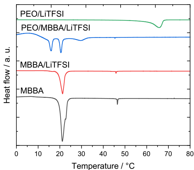
Fig. 2 Differential scanning calorimetry thermograms of PEO/LiTFSI (green), PEO/MBBA/LiTFSI (blue), 0.5 M solution of LiTFSI in MBBA (red) and MBBA (black)
