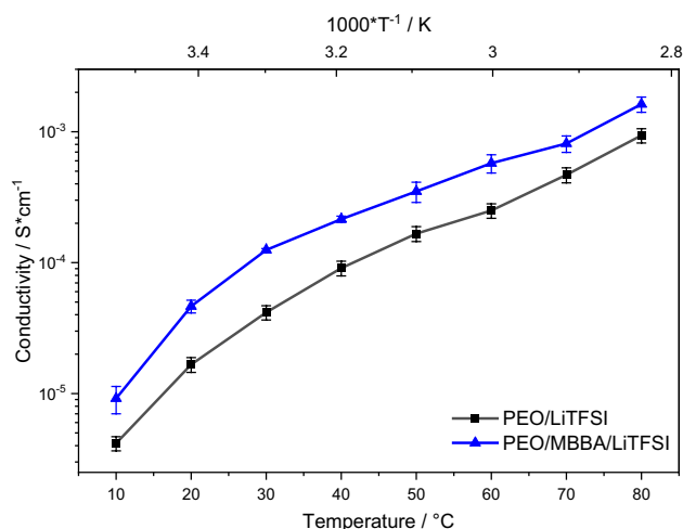
Fig. 3 Ionic conductivity of PEO/LiTFSI (black) and PEO/MBBA/LiTFSI (blue) solid polymer electrolytes as a function of the temperature
