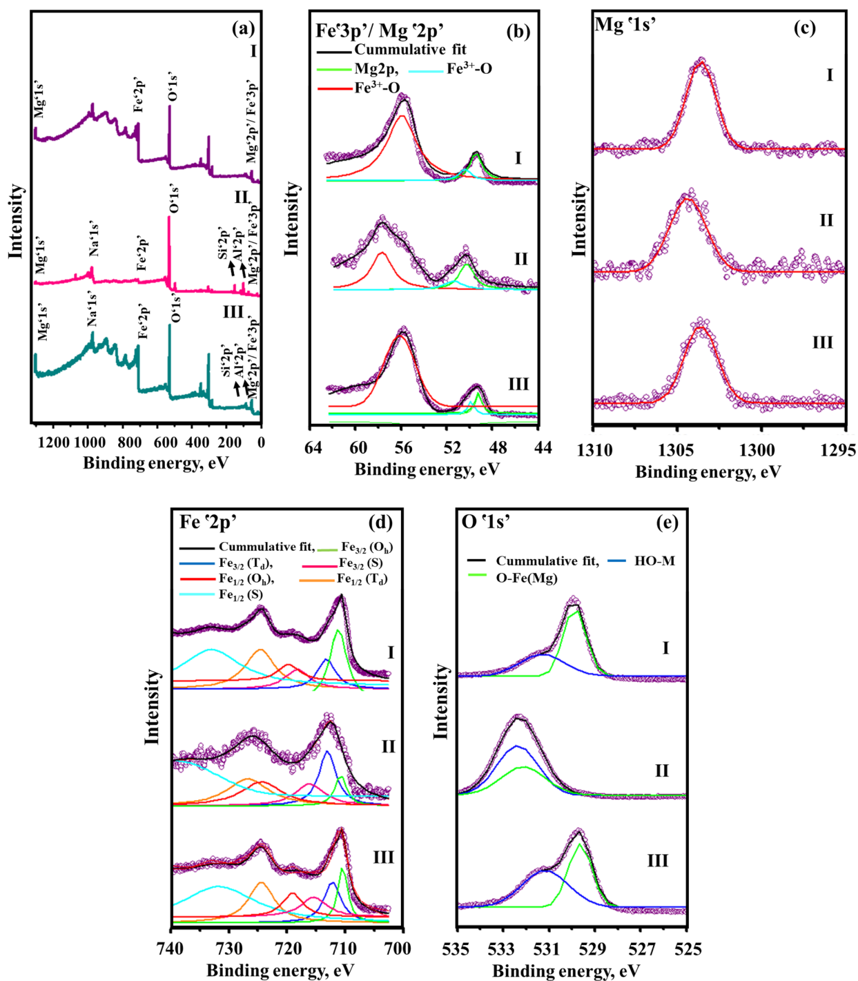
Figure 1: (a) Full survey spectrum and XPS high-resolution spectra of (b) Mg 2p /Fe 3p , (c) Mg 1s , (d) Fe 2p , and (e) O 1s of MgFe 2 O 4 (I), bentonite (II), and MgFe 2 O 4 -bentonite (III).
