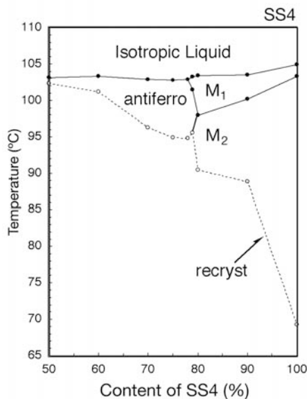
Figure 1. Phase diagram between chiral molecule SS 4 and the racemic mixture ( SS 4 :RR 4 = 1:1). Reprinted in part with permission from Chem. Mater. 16 (17) (August 24, 2004) p. 3213. ©2004 American Chemical Society.
