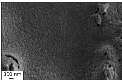
Figure 2. Surface of converted and hydroxyapatite-coated coral. The micro- and nanopores of the converted coral are covered with a sol-gel-derived hydroxyapatite layer.
