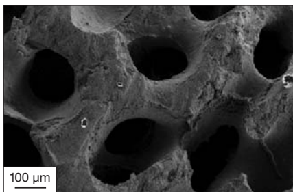
Figure 1. Surface of coral containing interconnected macropores of 150–500 \mu\text{m} .
