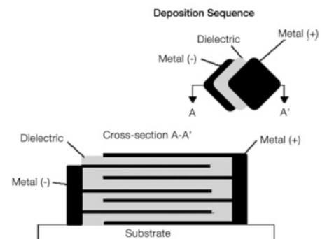
Figure 1. Idealized aspects of a multilayered capacitor design, showing the alternating metal and dielectric laminations and a cross section of the multilayered capacitor. The total height, including the substrate, will be less than 0.5 mm.
