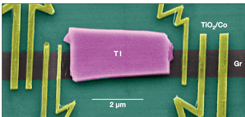
Scanning electron microscope image of the Dirac material heterostructure. TI is topological insulator. Credit: Science Advances , AAAS.
