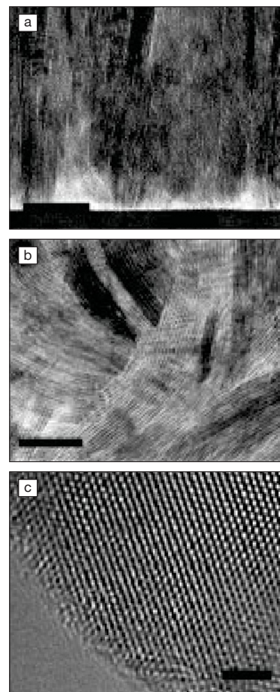
(a) Cross-sectional transmission electron microscope (TEM) image of \text{MoS}_2 thin film (scale bar = 20 nm); (b) plan-view TEM image of \text{MoS}_2 thin film (scale bar = 10 nm); and (c) bulk \text{MoS}_2 crystal (scale bar = 2 nm). Credit: Zhu et al.
