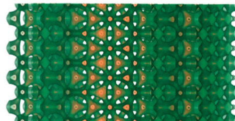
An extrinsic stacking fault in hexagonally close-packed magnesium. Defects at the atomic scale, which are revealed in the electronic structure shown here, affect the macroscopic mechanical properties such as the elastic and plastic deformation. Credit: W.Y. Wang and Z.K. Liu: private communication.
