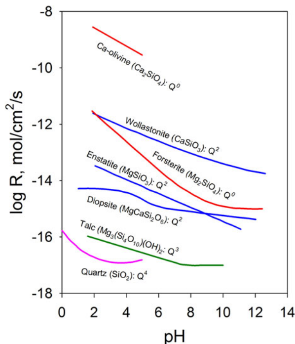
Figure 1: Dissolution rate of Ca/Mg silicates at 25 °C as a function of pH (enstatite at 70 °C) and the connectivity of [SiO 4 ] tetrahedrons. Data are from Ref. 10 and the references therein. The rate is the forward rate.
