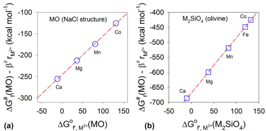
Figure 5: A graphic representation of Eq. (5) rearranged to \Delta G_{f, M^{2+}}^{\#} - \beta^{\#} r_{M^{2+}}^{\#} = a^{\#} \cdot \Delta G_{f, M^{2+}}^{\circ} + b^{\#} . Effective free energy for the formation of surface complexes on metal oxides with rock salt structures (a) and orthosilicates with olivine structures (b). The symbols are calculated from experimental data. The dashed lines are regression lines. Adapted from Ref. 86.
