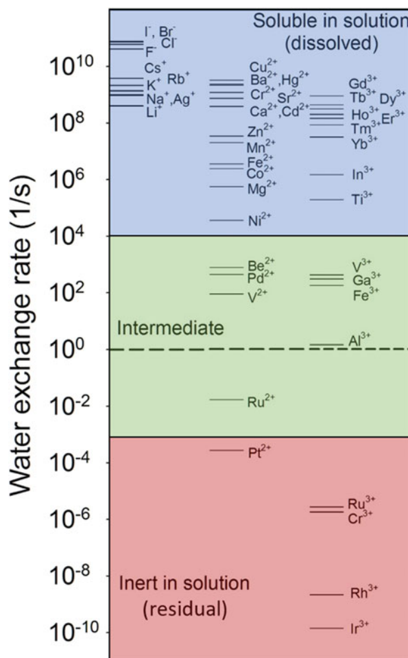
Figure 2: Water-exchange rate constant for a particular water molecule in the first coordination sphere of aqueous ion [\text{M}(\text{H}_2\text{O})_n]^{m+} . Data are from Ref. 78. The dashed line refers to the exchange rate of 1 \text{ s}^{-1} .
