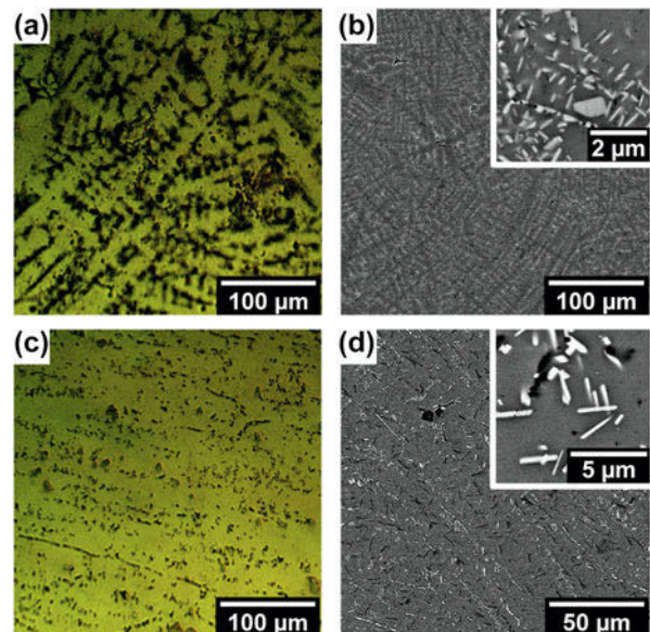
Figure 4: Microstructure of the 1-h annealed sample in (a) optical micrograph and (b) SEM-BSE micrograph; and 24-h annealed sample in (c) optical micrograph and (d) SEM-BSE micrograph.
