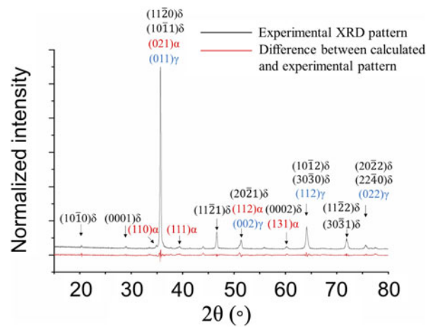
Figure 3: XRD patterns and refinement for the 24-h annealed sample.
