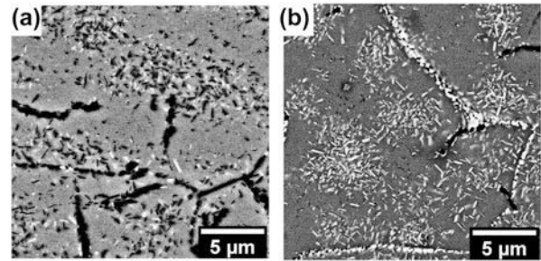
Figure 2: SEM-BSE micrographs of samples electrolytic polished at (a) room temperature and (b) -20 °C.
