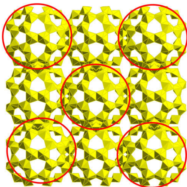
FIG. 1. One unit cell (a 5 37.884 Å, from the [100] direction) of the U_{60} -bearing crystalline compound: Li_{68}K_{12}(OH)_{20}[UO_2(O_2)(OH)]_{60}(H_2O)_{310} with Li, K, and H_2O omitted for clarity. Cluster molecules circled are in-plane with the page.
