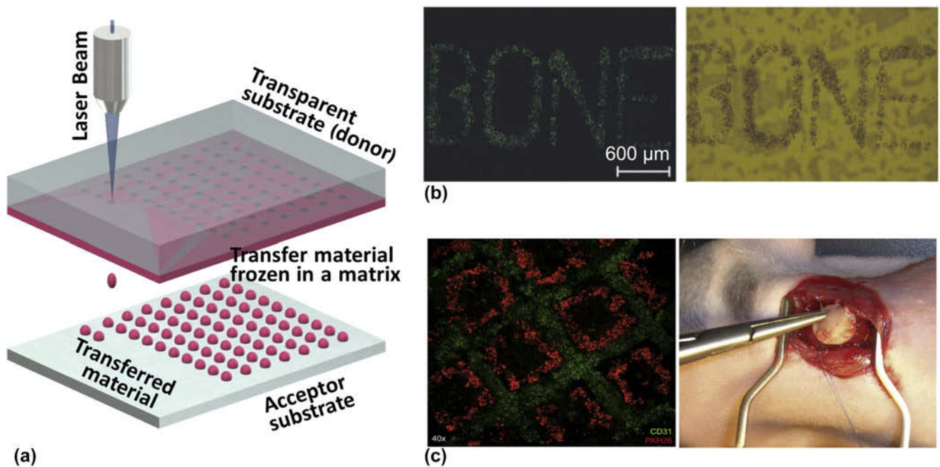
FIG. 3. Laser induced forward transfer (LIFT) for biofabrication (a) schematic of LIFT technology; (b) mesenchymal stem cells were patterned into “BONE” using LIFT technology with high cell viability 66 ; and (c) human umbilical vein endothelial cells and mesenchymal stem cells were co-patterned by LIFT technology on a cardiac patch, which was implanted in vivo onto the area of blanched myocardium. 70
