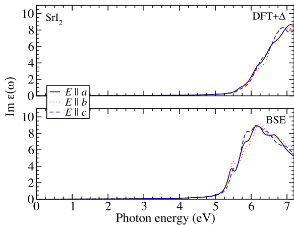
FIG. 5. Imaginary part of the dielectric function \varepsilon(\omega) computed using the DFT + \Delta approximation (top) as well as the BSE approach (bottom) for SrI 2 . The optical anisotropy is shown for both.
