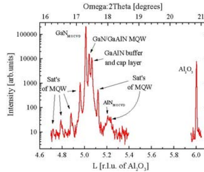
Figure 2. Reciprocal lattice scan of GaAlN/GaN MQW along growth axis. Satellites of the superlattice corresponding to the MQW section allow to calculate thickness of each layer. Measurement was performed in reciprocal lattice units of sapphire.
