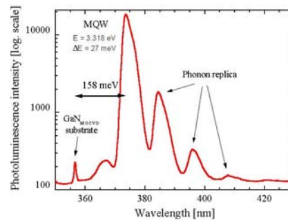
Figure 3. Low temperature photoluminescence spectra of multi-quantum well.
