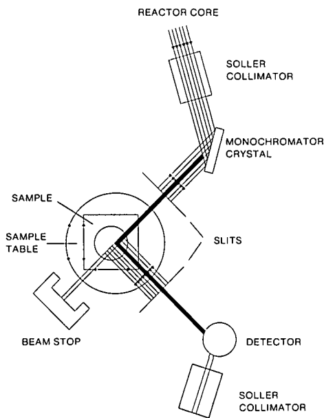
Schematic of Chalk River's residual strain measurement using slits to define a small beam. After a beam of polychromatic neutrons is extracted from the reactor core, a monochromatic beam is obtained. The slits define a narrow beam which usually passes through the sample and reaches the beam stop. A slit is placed in the diffracted beam from which all the diffracted information originates. (From Ref. 2, Nov. 1986.)
