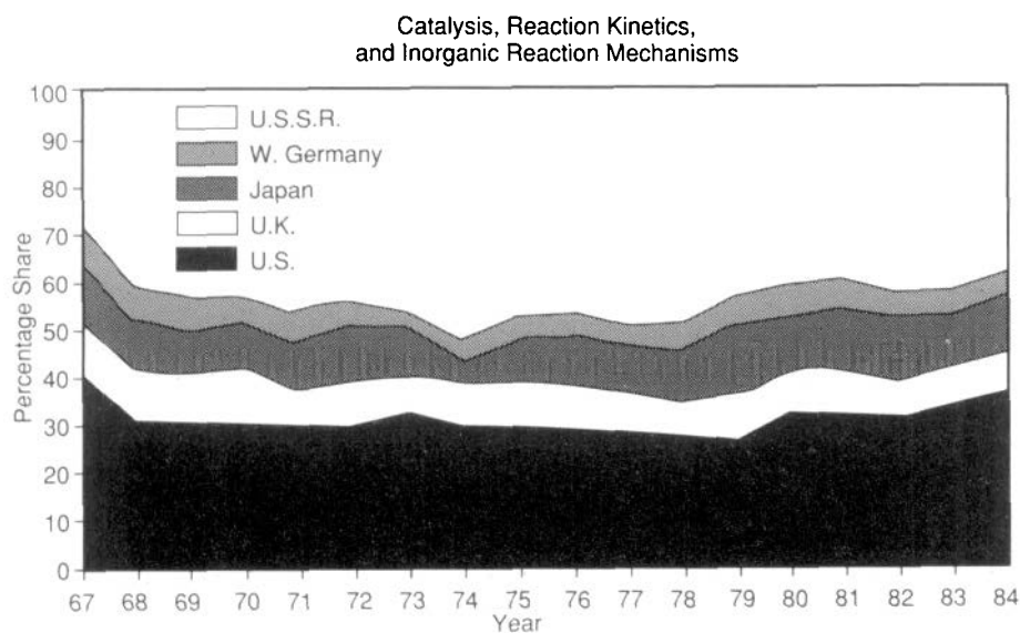
Figure 1. Production of papers in catalysis, reaction kinetics, and inorganic mechanisms research; relative contributions of six countries.
