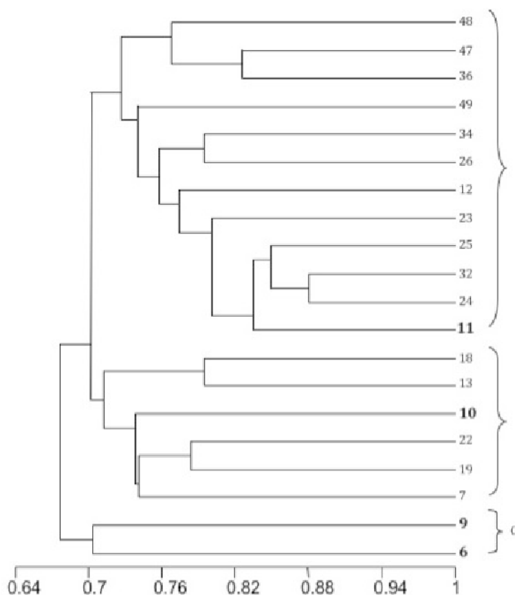
Figure 2. SSR based cluster formation of 20 genotypes of the B-genome synthetic hexaploids ( 2n = 6x = 42 ; AABB 5 B/SS)
