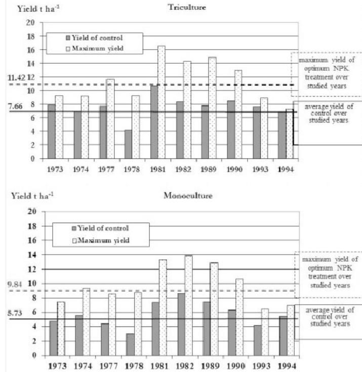
Figure 2. Effect of crop rotation and fertilization on the yield of maize (Hajdúböszörmény, 1973–1994)
