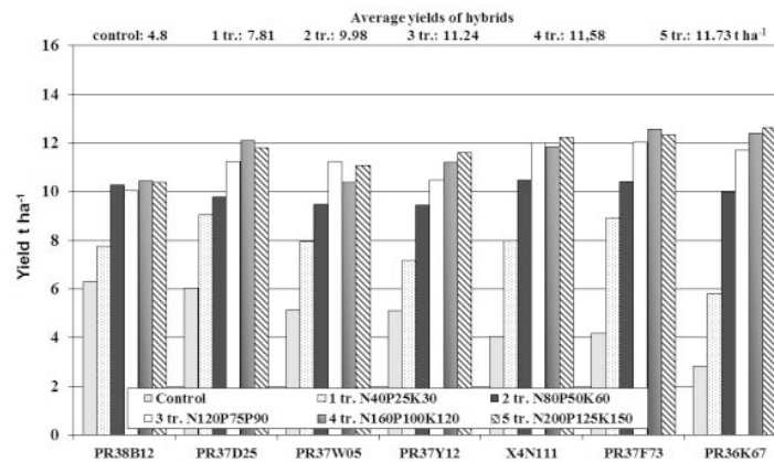
Figure 3. The effect of fertilization on hybrid maize yields (Hajdúböszörmény, 2006) (LSD 5% Hybrid = 0.54 t ha -1 ; Plants = 0.53 t ha -1 ; Reciprocal effect = 1.39 t ha -1 )
