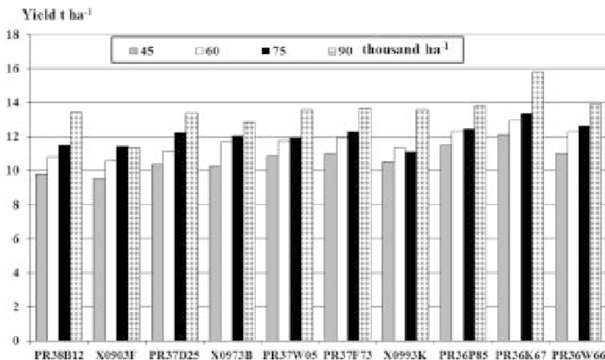
Figure 5. Effect of plant density on maize hybrid yields (Hajdúböszörmény, 2005) (LSD 5% Hybrid = 0.87 t ha -1 ; Plants = 0.48 t ha -1 ; Reciprocal effect = 1.51 t ha -1 )
