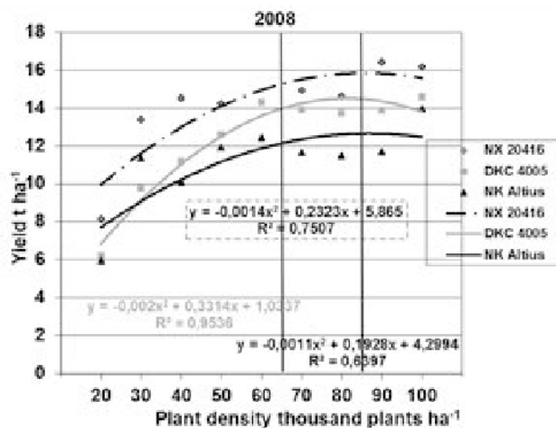
Figure 4. The effect of plant density on the yield of maize (Hajdúböszörmény, 2008) (LSD 5% Hybrid = 0.97 t ha -1 ; Plants = 0.26 t ha -1 ; Reciprocal effect = 1.26 t ha -1 )
