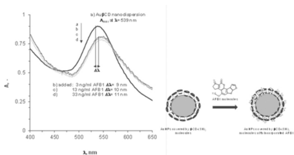
Figure 3. Absorbance spectra of Au \beta CD nanodispersions added AFB1 and schematic presentation of AuNPs covered by \beta CD-(SH) 2 before and after incorporation of AFB1 molecules
