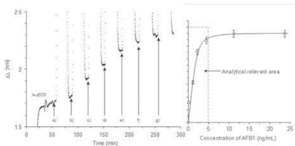
Figure 4. SPR curve of AFB1 (b) 1, c) 5, d) 10, e) 30, f) 60 pg/ml) on a) Au \beta CD NPs modified surface measured on SPR platform, and adsorption isotherm of AFB1 on Au \beta CD NP-modified Au film measured on SPR platform
