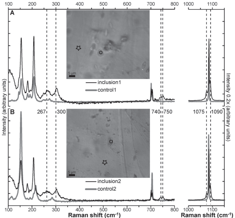
Fig. 3. Raman spectra obtained from inclusions and host aragonite. Analyses performed on inclusions and adjacent, inclusion-free control spots at two selected sectors of an eel otolith (MT18 in Tab. 1) (A, B). Investigated sectors with numerous fusiform inclusions viewed in transmitted light are shown as inset image above the corresponding Raman spectra. For better visualization, the spectra beyond 1000 \text{ cm}^{-1} are scaled to 0.2\times in intensity. Analysed spots are marked with circle (inclusion) and star (host aragonite) in the images. Characteristic Raman bands for vaterite, marked by dashed vertical lines, and corresponding wavenumbers are indicated. The vaterite signal was only observed from the inclusions. Note that the Raman spectra from inclusions show bands of both vaterite and aragonite because the confocal settings and inclusion dimensions did not allow a complete elimination of the host aragonite signal
