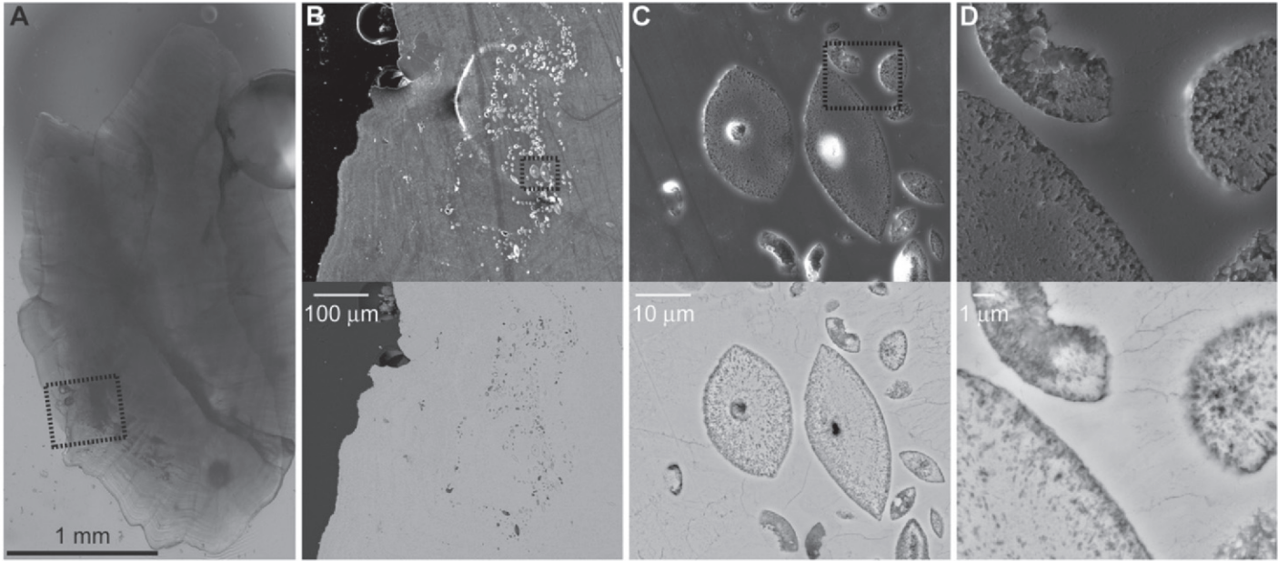
Fig. 1. Microscopic view of a polished eel sagitta with abundant inclusions. (MT1 in Tab. 1) A: Inclusion-rich zones appear as dark clouds within the transparent host matrix as viewed in transmitted light. B–D: Magnification series of scanning electron micrographs showing the (micro)texture of the new morphological type of inclusions. Secondary and backscattered electron images are shown in the top and bottom, respectively. Dashed squares indicate the magnified area
