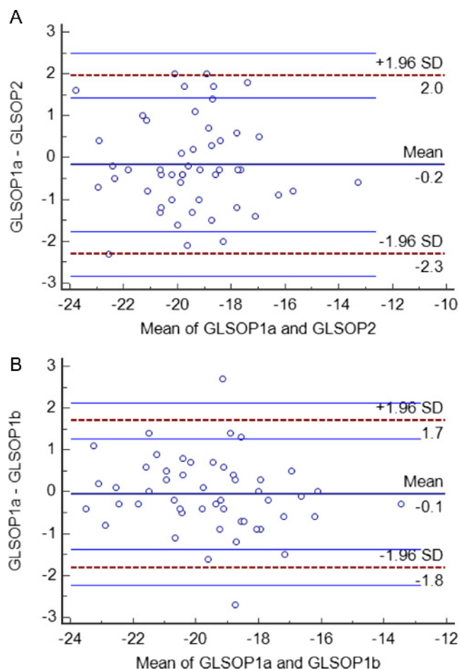
Figure 2 Bland-Altman plots showing inter-operator and intra-operator measurement of GLS.
