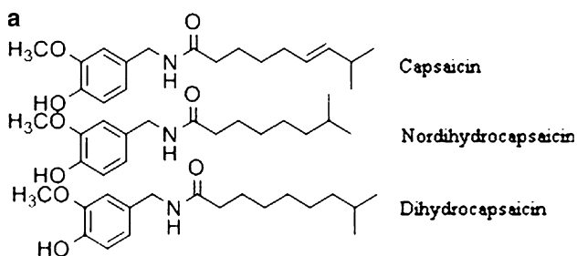
Fig. 1. a Structures of capsaicinonids
