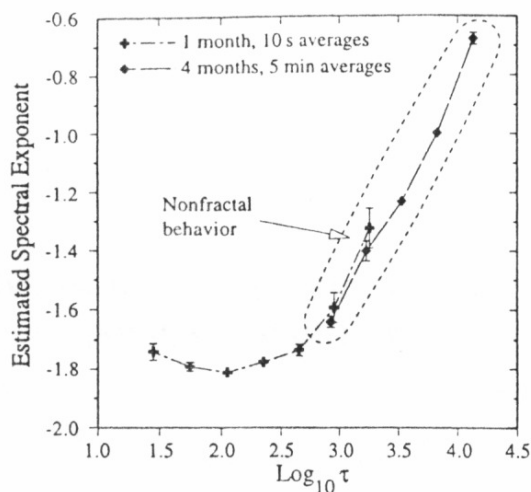
Figure 55: Spectral exponents for the B_z component estimated from the length function computed from Ulysses magnetic field data, when the s/c was at about 4 AU and \sim -50^\circ latitude. Different symbols refer to different time intervals as reported in the graph. Image reproduced by permission from (from Horbury et al. , 1995a).
