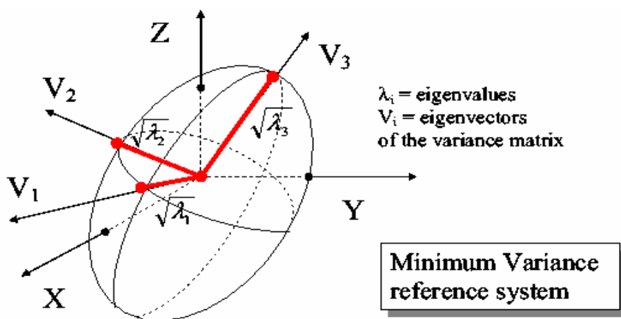
Figure 119: Original reference system [x, y, z] and minimum variance reference system whose axes are V_1, V_2, and V_3 and represent the eigenvectors of M . Moreover, \lambda_1, \lambda_2, and \lambda_3 are the eigenvalues of M .
