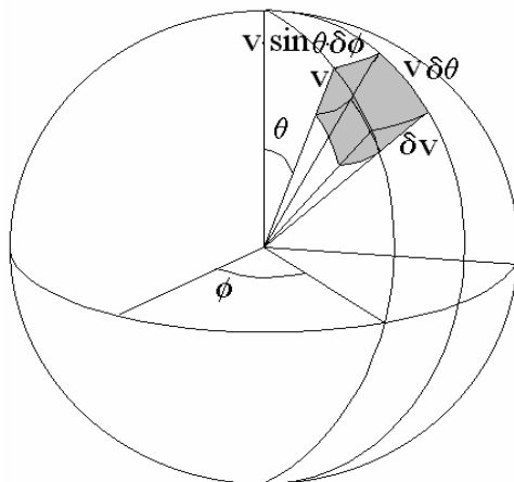
Figure 122: Unit volume in phase space.
