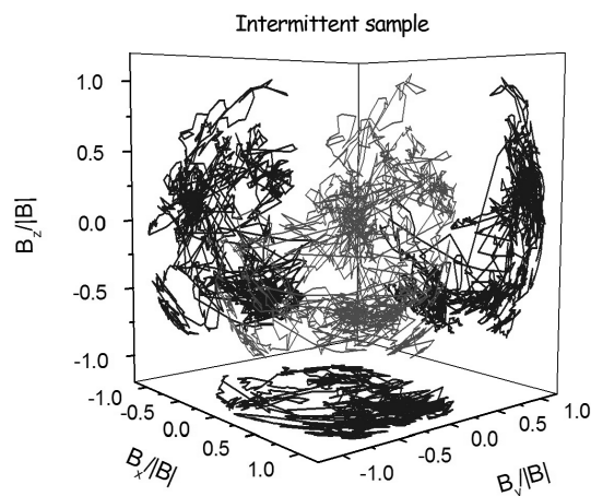
Figure 100: Still from a movie showing Trajectory followed by the tip of the magnetic field vector in the minimum variance reference system during a time interval characterized by intermittent events. The duration of the interval is 2000 \times 6 s but the magnetic field vector moves only for 100 \times 6 s in order to make a smaller file (movie kindly provided by A. Vecchio). (To watch the movie, please go to the online version of this review article at http://www.livingreviews.org/lrsp-2013-2 .)
