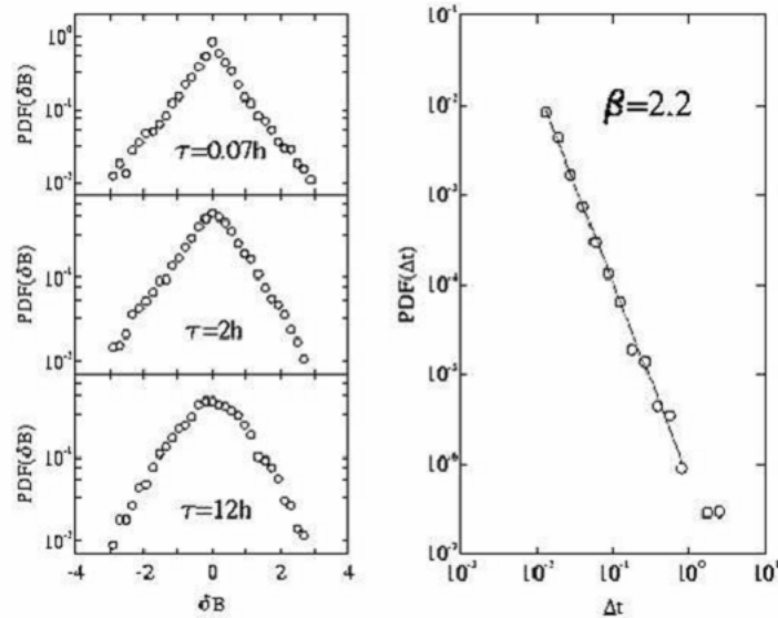
Figure 82: Left panel: normalized PDFs for the magnetic fluctuations observed in the solar wind turbulence by using Helios data. Right panel: distribution function of waiting times \Delta t between structures at the smallest scale. The parameter \beta is the scaling exponent of the scaling relation \text{PDF}(\Delta t) \sim \Delta t^{-\beta} for the distribution function of waiting times.
