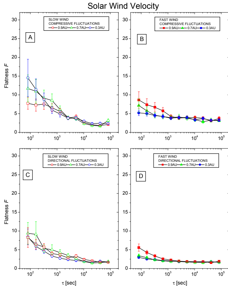
Figure 107: Flatness \mathcal{F} vs. time scale \tau relative to wind velocity fluctuations. In the same format of Figure 106 panels A and C refer to slow wind and panels B and D refer to fast wind. The upper panels refer to compressive fluctuations and the lower panels refer to directional fluctuations. Vertical bars represent errors associated with each value of \mathcal{F} . Image reproduced by permission from Bruno et al. (2003b), copyright by AGU.
