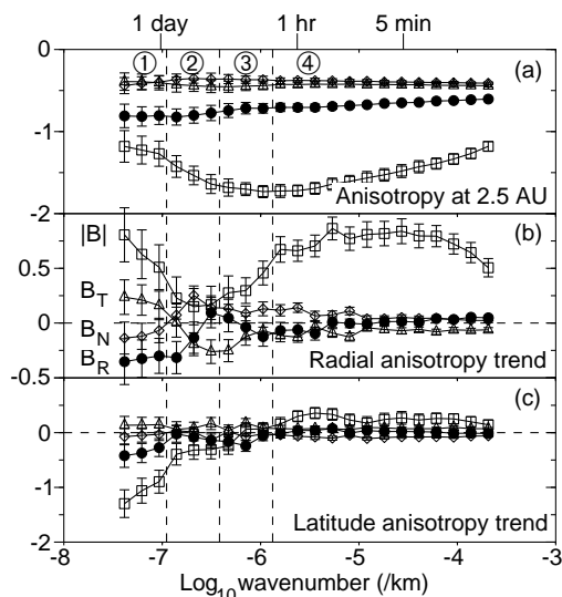
Figure 59: (a) Scale dependence of power anisotropy at 2.5 AU plotted as the \log_{10} of the ratio of B_R (solid circles), B_T (triangles), B_N (diamonds), and |\mathbf{B}| (squares) to the trace of the spectral matrix; (b) the radial, and (c) latitudinal behavior of the same values, respectively. Image reproduced by permission from Horbury and Balogh (2001), copyright by AGU.
