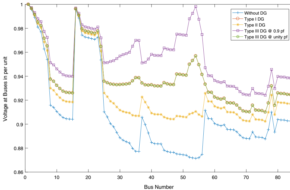
Fig. 9 Voltage profile of 69-bus system
