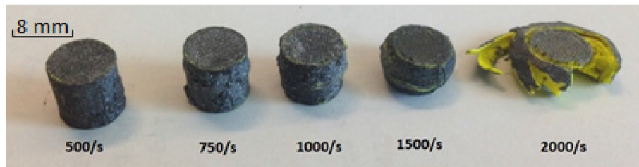
Fig. 10 Specimen deformation
