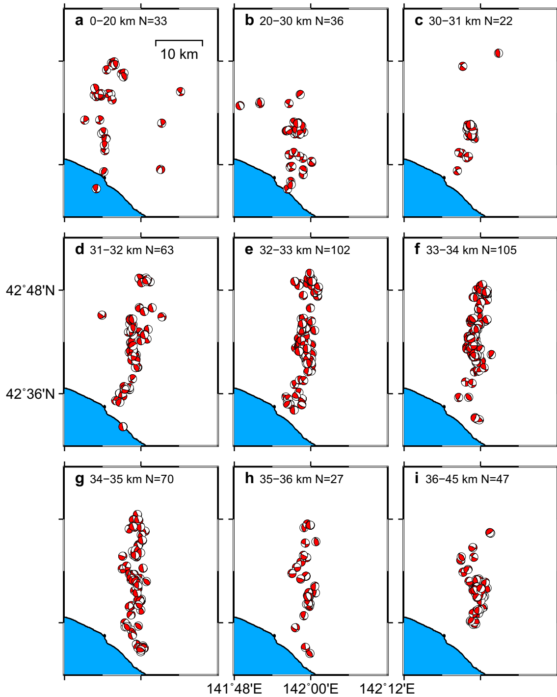
Fig. 4 Focal mechanism solutions with Quality A and B determined in this study. The depth of hypocenter is a 0–20 km, b 20–30 km, c 30–31 km, d 31–32 km, e 32–33 km, f 33–34 km, g 34–35 km, h 35–36 km, and i 36–45 km. All diagrams are equal area projections on the lower hemisphere of the focal sphere. Colored areas show compressional quadrants
