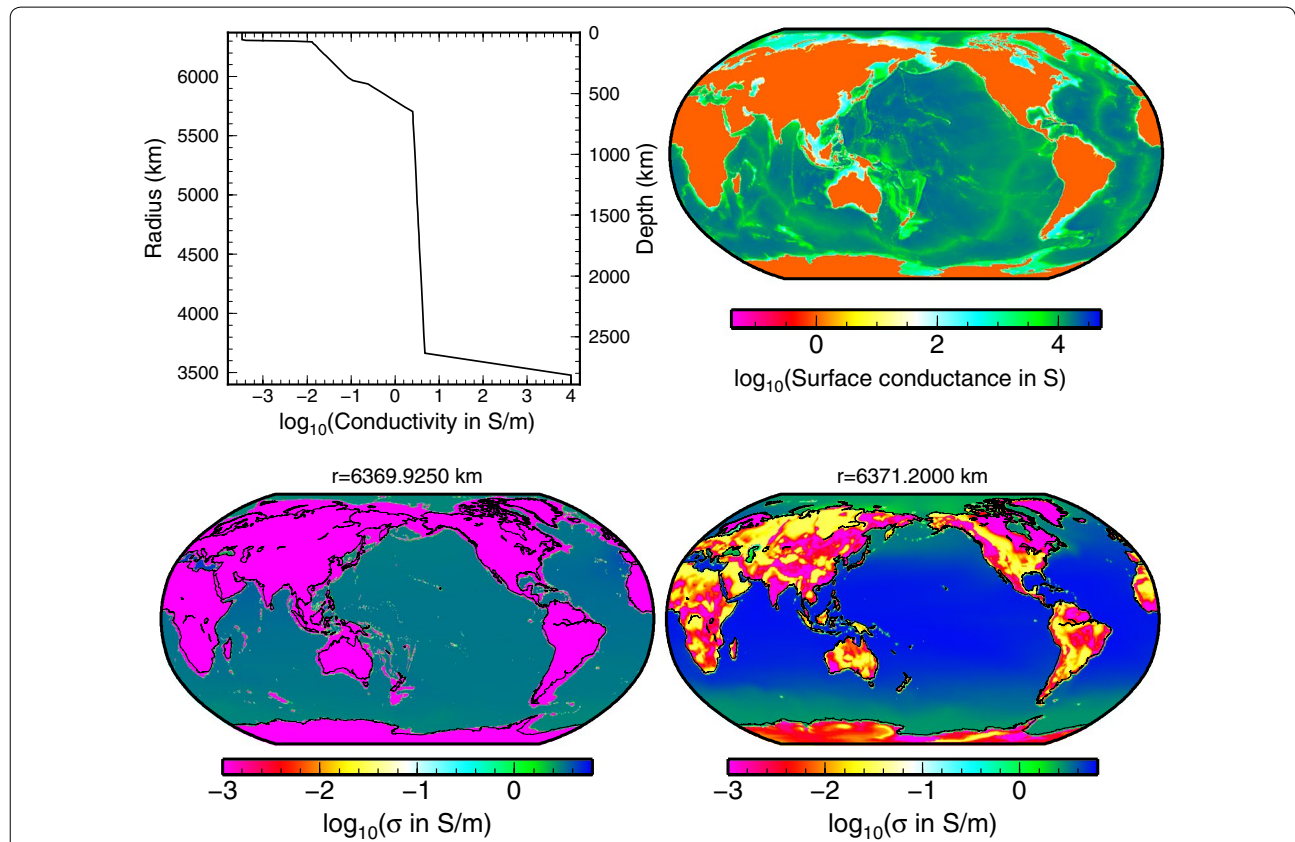
Fig. 2 Electrical conductivity. Top left: The 1-D electrical conductivity profile of the Earth’s mantle after Grayver et al. (2017). Top right: Map of the electrical surface conductance of the oceans and continents used in the 2-D models. Bottom: Electrical conductivity map including the effects of seawater salinity, temperature, and the presence of sediments. Cross sections at 1.275 km depth (left) and at the surface (right)
